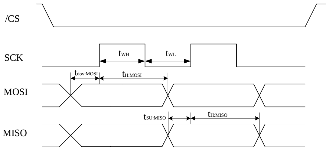
SPI timing
