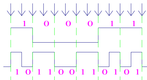
Figure 7.2. Biphas-Mark Encoding
