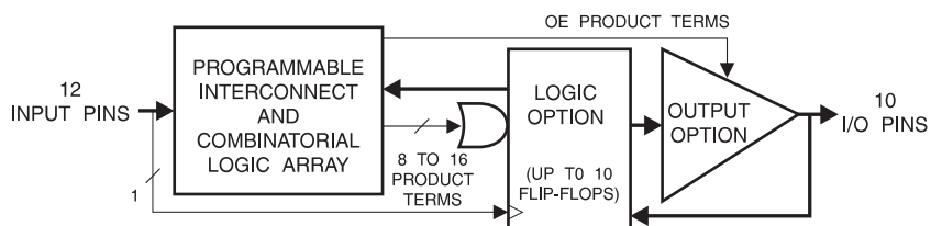
Figure 1-1. Block Diagram
