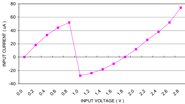
INPUT CURRENT VS. INPUT VOLTAGE INPUT PIN ( V_{CCINT} = 1.8V , T_A = 25^\circ C ) (PIN-KEEPER ON)
