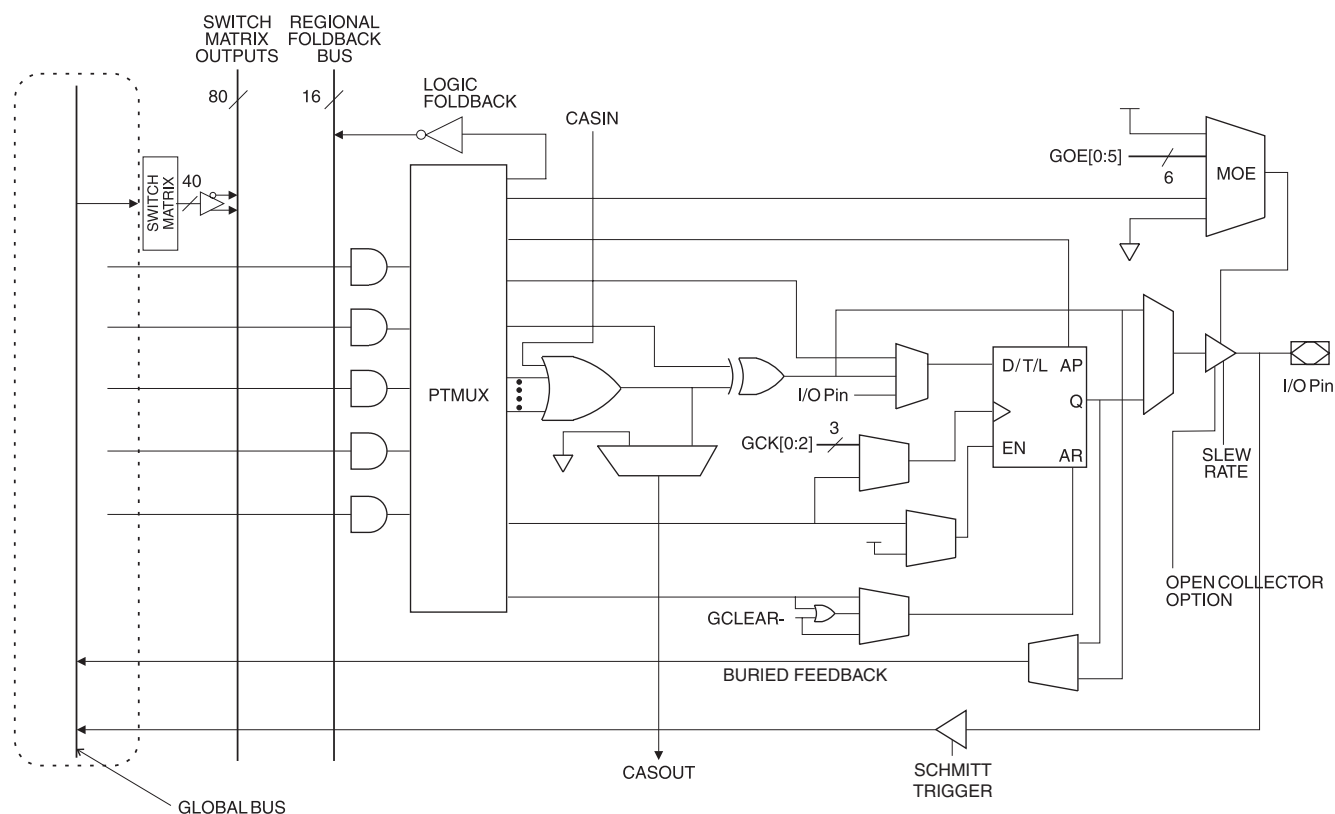
Figure 1-4. ATF1504BE Macrocell
