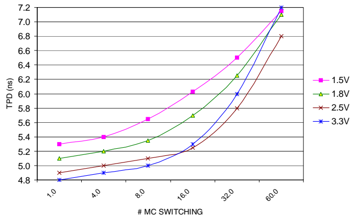
TPD VS. # MC SWITCHING ( V_{CCINT} = 1.8V , V_{CCIO} = 1.5-3.3V , T_A = 25^\circ C )
