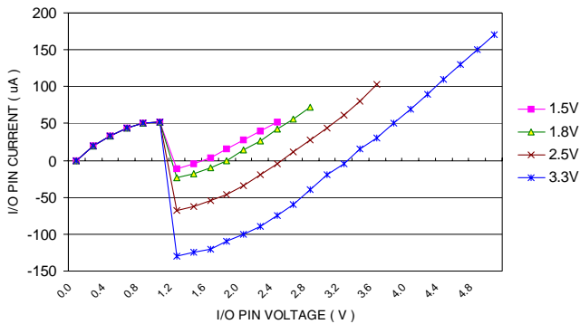
I/O PIN CURRENT VS. I/O PIN VOLTAGE I/O PIN ( V_{CCINT} = 1.8V , V_{CCIO} = 1.5V-3.3V , T_A = 25^\circ C ) (PIN KEEPER ON)
