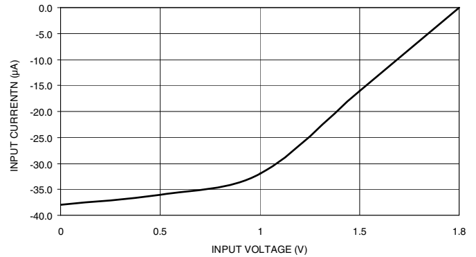
INPUT & I/O CURRENT VS. INPUT VOLTAGE V_{CCINT} = 1.8V , V_{CCIO} = 1.8V ( T_A = 25^\circ C ) (Pull-Up On)
