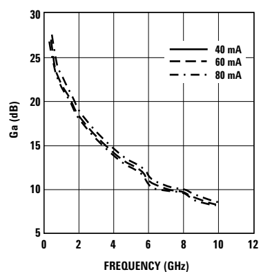
Figure 11. Ga vs. Frequency vs. I_{ds} , V_{ds} = 3V^{[1]} .
