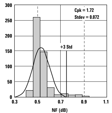
Figure 4. NF @ 2 GHz, 3 V, 60 mA. Nominal = 0.5, USL = 0.9
