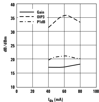
Figure 8. Gain, OIP3 & P1dB vs. I_{ds} Tuned for Max OIP3 and Min NF at 2 GHz, V_{ds} = 3V^{[2]} .
