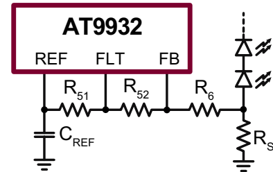
Figure 5. Output Short Circuit Protection
