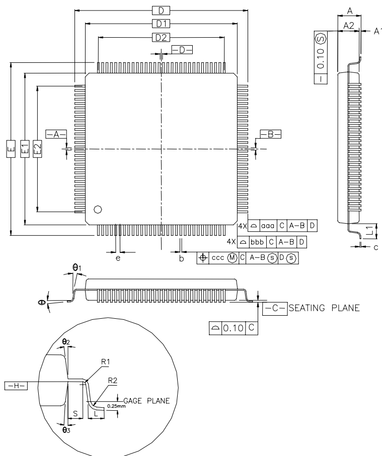
Figure 11-1. 208-pin PQFP Package Drawing
