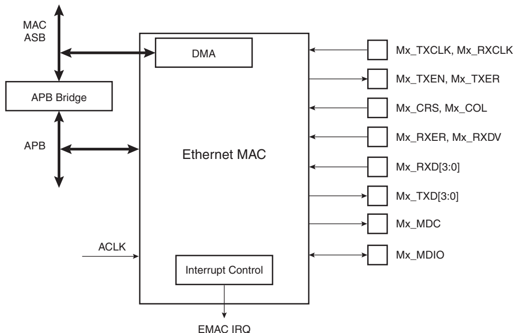
Figure 16-1. Block Diagram
