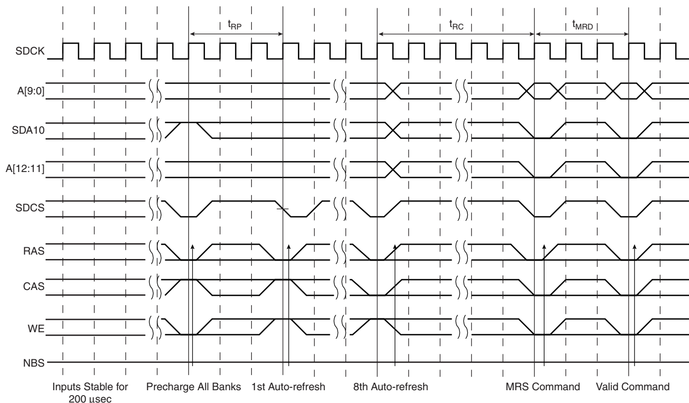
Figure 14-3. SDRAM Device Initialization Sequence
