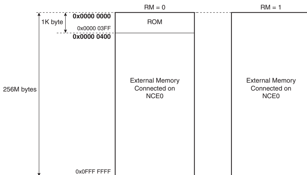
Figure 9-4. ROM Mapping Depending on the Boot Mode
