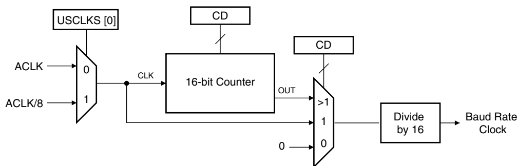
Figure 19-2. Baud Rate Generator
