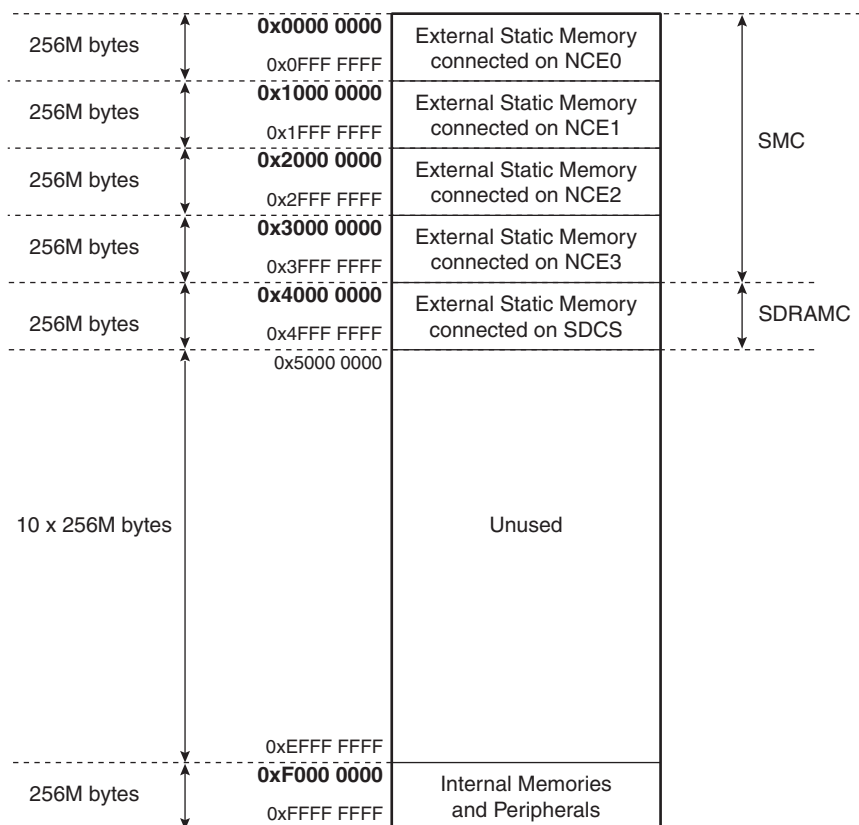
Figure 9-2. AT91C140 Memory Map
