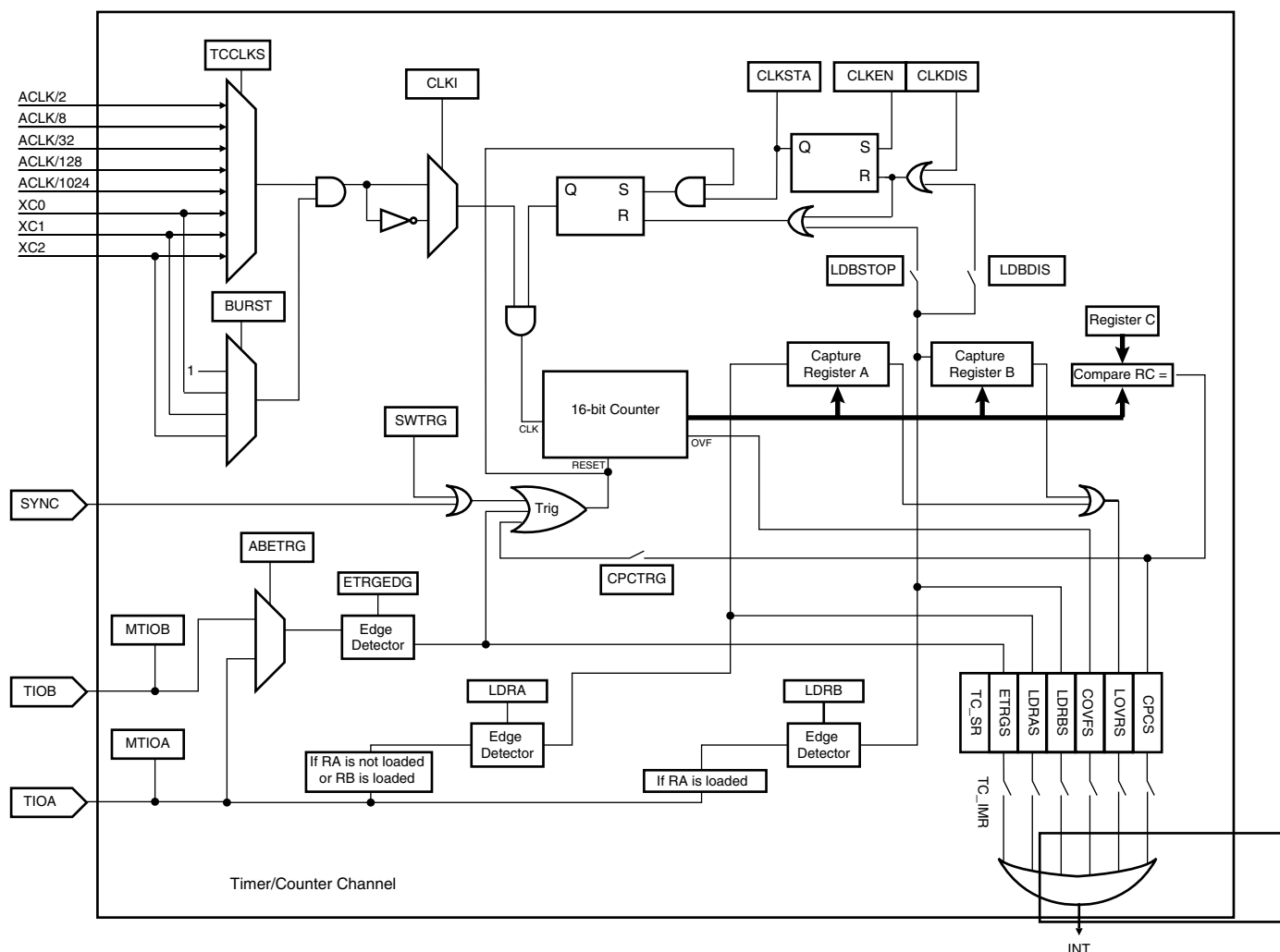
Figure 20-4. Capture Mode
