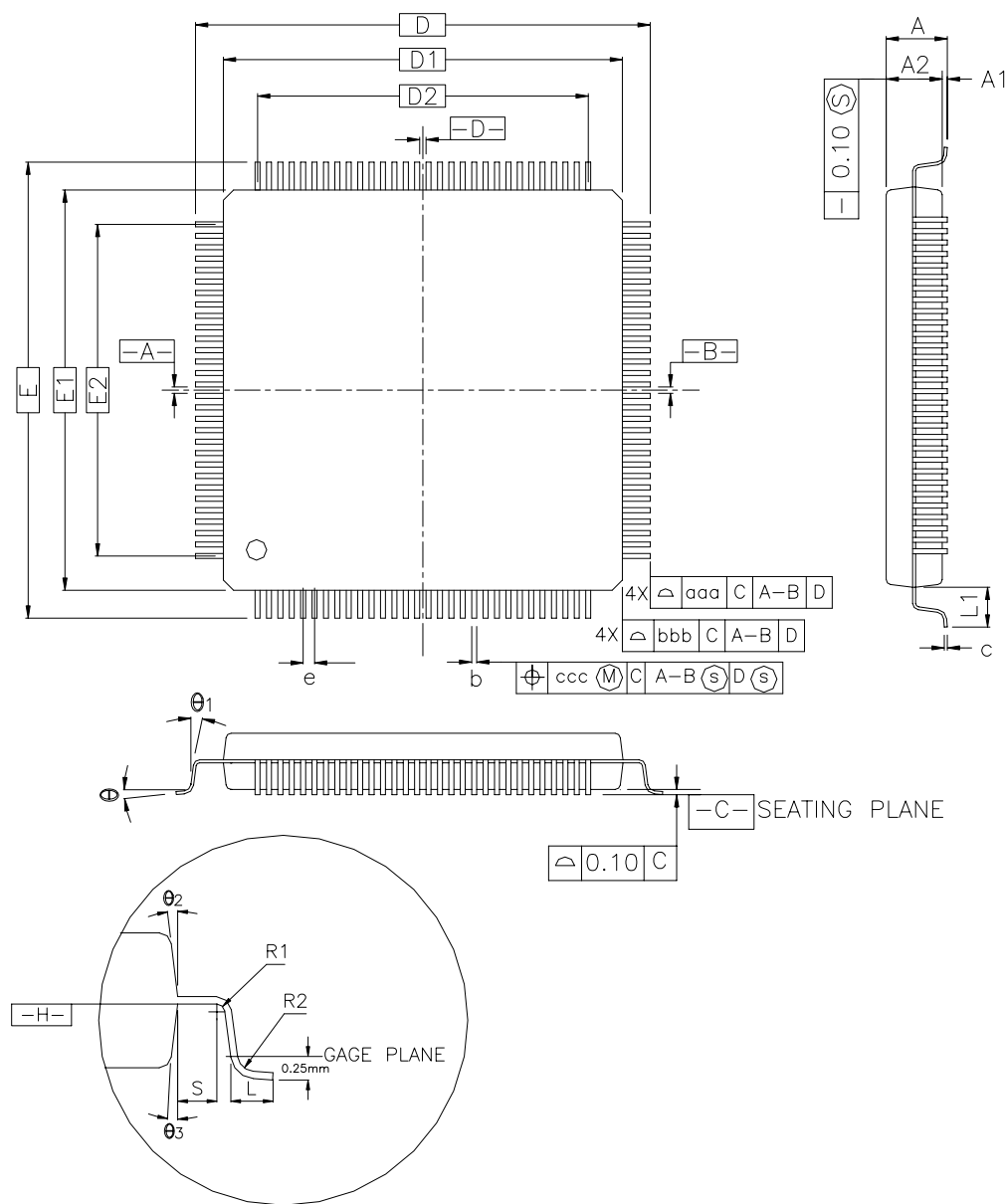
Figure 22-1. AT91C140 PQFP Package
