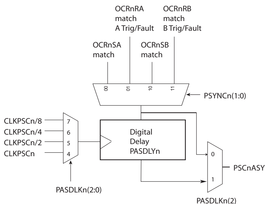
Figure 12-40. Analog synchronization.
