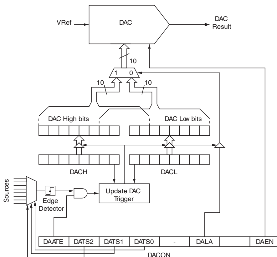
Figure 18-1. Digital to analog converter block schematic.
