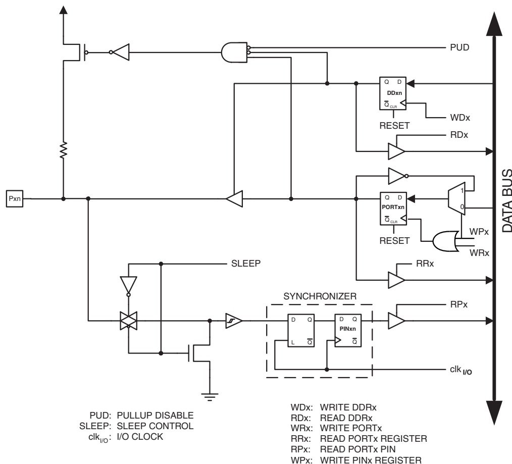
Figure 9-2. General digital I/O (1) .
