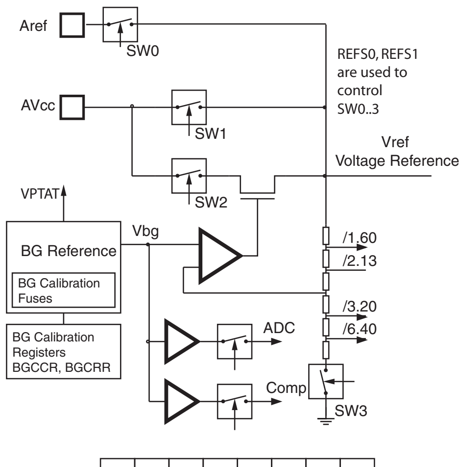
Figure 15-1. Reference circuitry.
