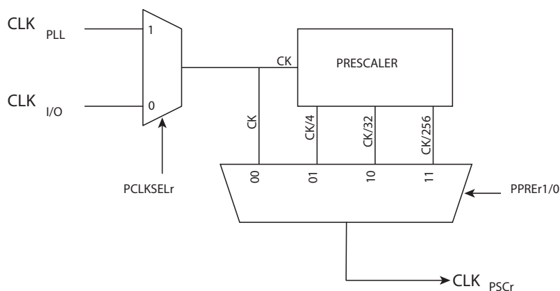
Figure 13-32. Clock selection.
