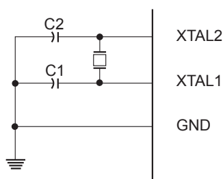
Figure 5-2. Crystal oscillator connections.
