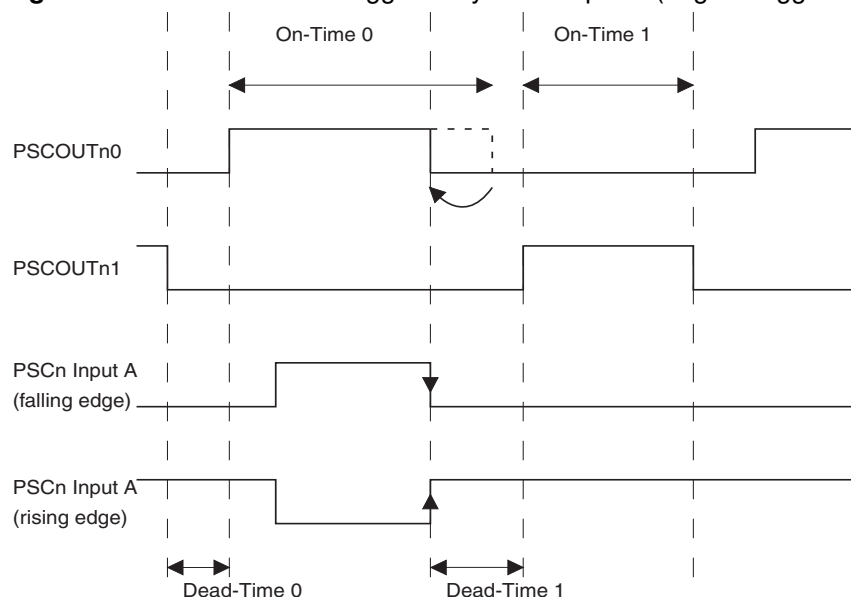
Figure 13-9. PSCOUTr0 retrigged by PSCr Input A (edge retrigging).
