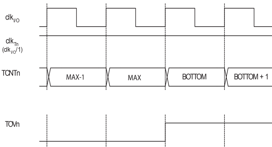
Figure 11-7. Timer/counter timing diagram, no prescaling.
