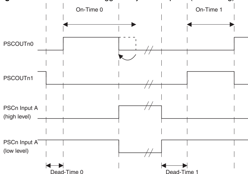
Figure 13-10. PSCOUTr0 retrigged by PSCr Input A (level acting).
