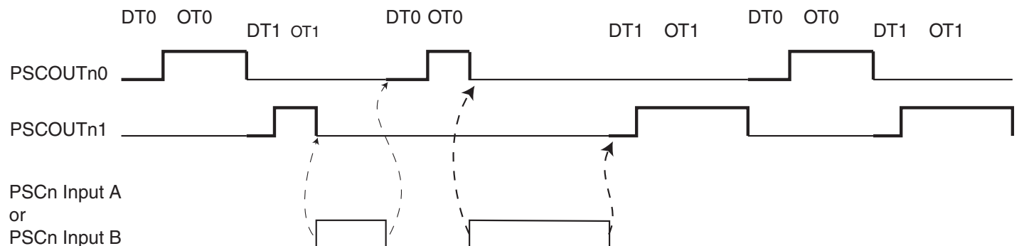
Figure 12-31. PSC behavior versus PSCn Input A in Fault Mode 6.
