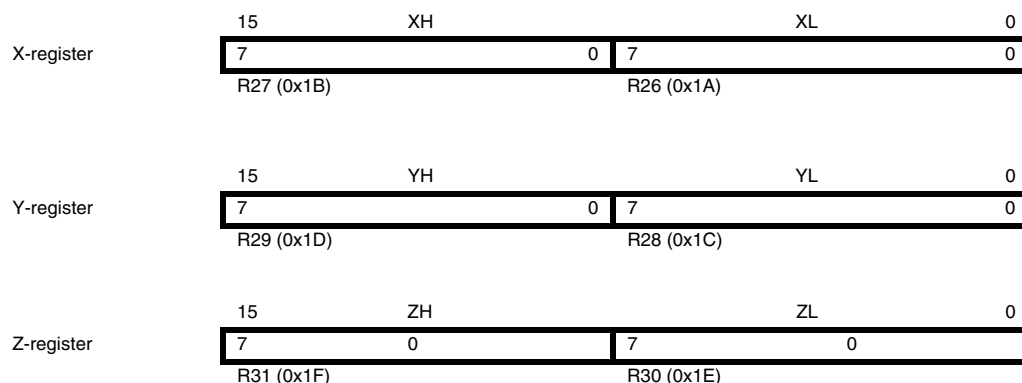
Figure 3-3. The X-register, Y-register, and Z-register.
