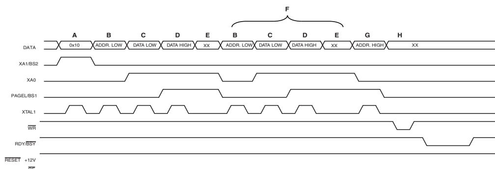
Figure 21-3. Programming the flash waveforms (1) .
