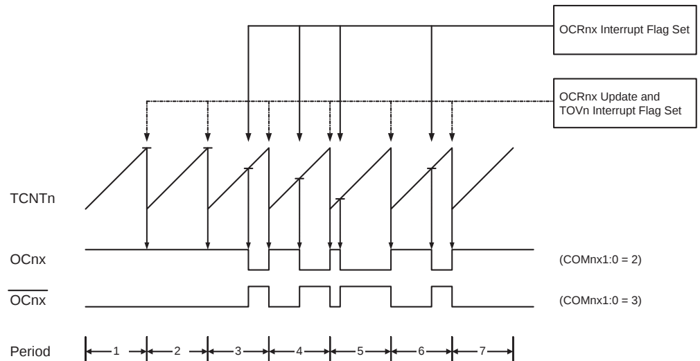
Figure 14-7. Fast PWM Mode, Timing Diagram
