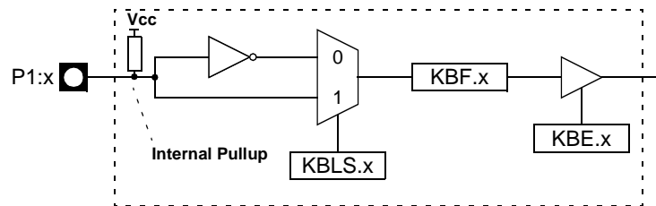
Figure 30. Keyboard Input Circuitry
