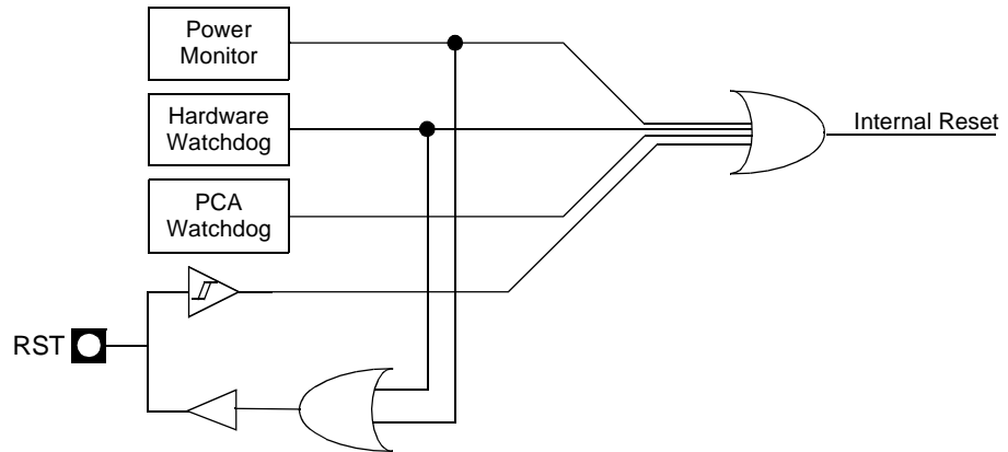
Figure 10. Reset Circuitry and Power-On Reset for AT89S54/58
