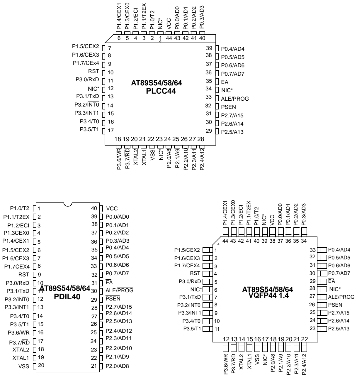
Figure 2. Pin Configurations
