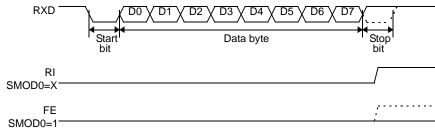
Figure 25. UART Timings in Mode 1
