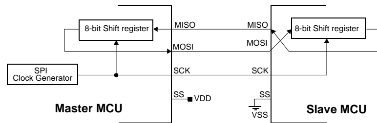
Figure 33. Full-Duplex Master-Slave Interconnection
