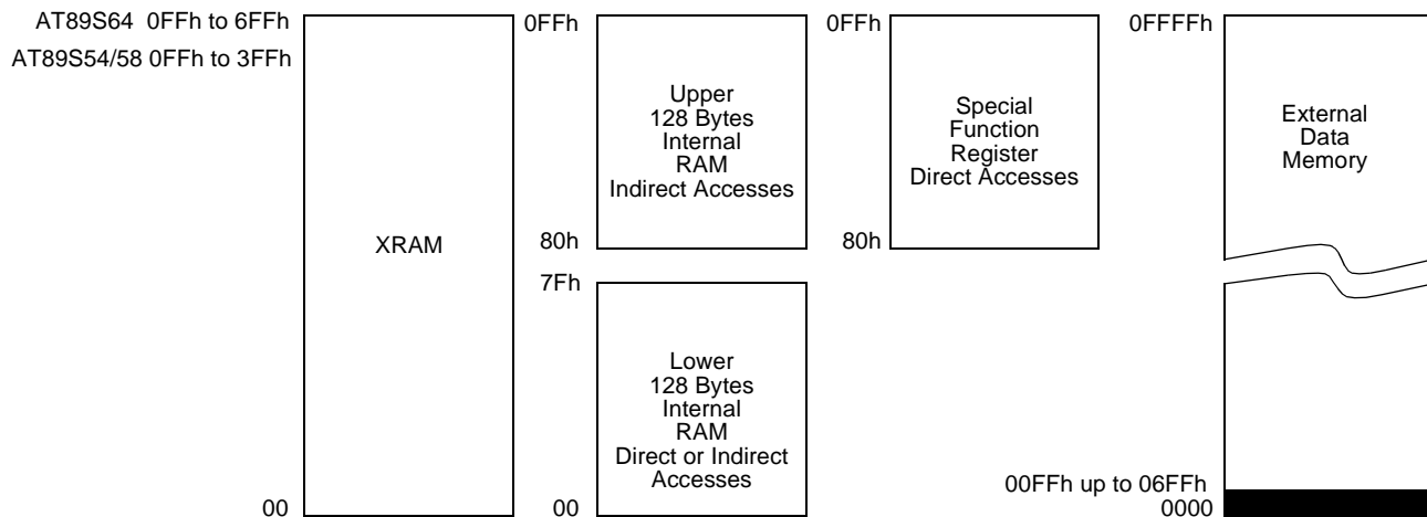
Figure 8. Internal and External Data Memory Address
