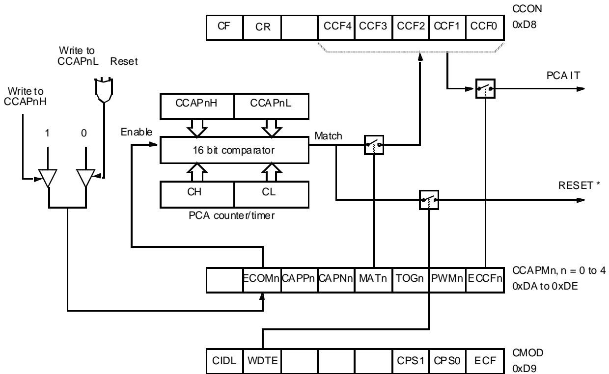
Figure 21. PCA Compare Mode and PCA Watchdog Timer
