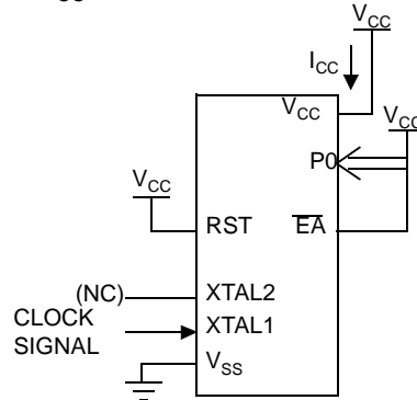
Figure 54. I_{CC} Test Condition, Active Mode
