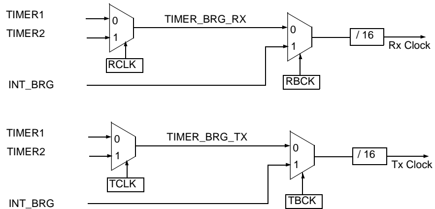
Figure 27. Baud Rate Selection
