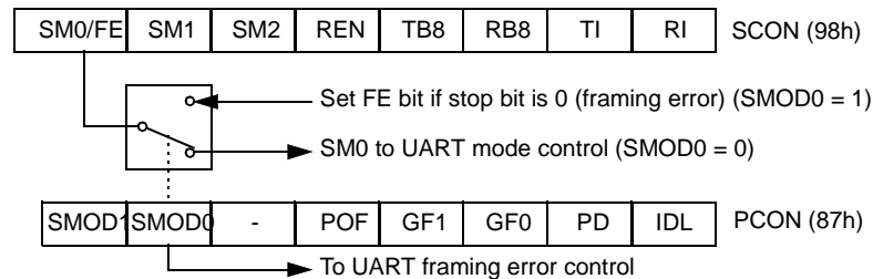
Figure 24. Framing Error Block Diagram
