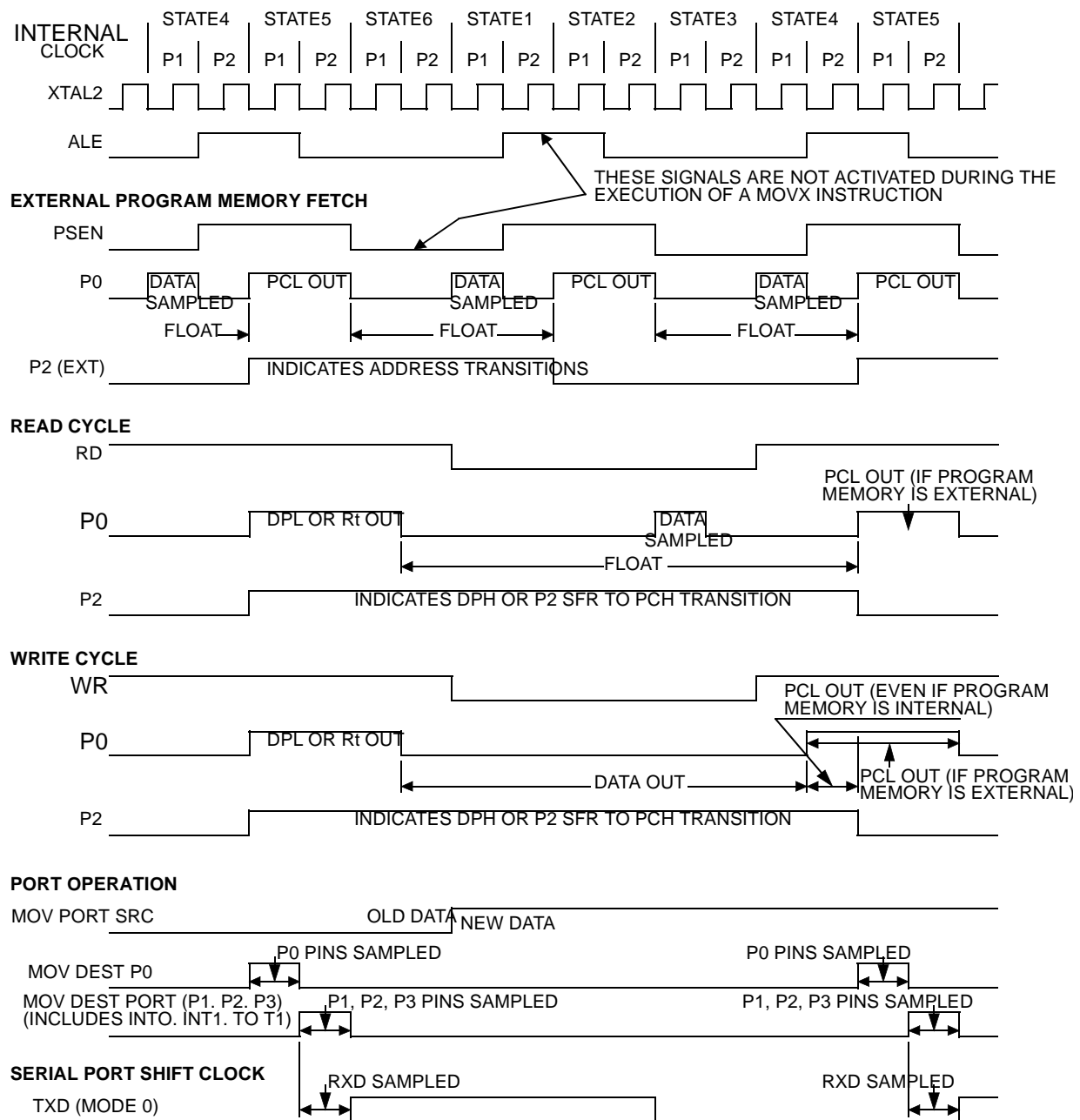
Figure 58. Internal Clock Signals
