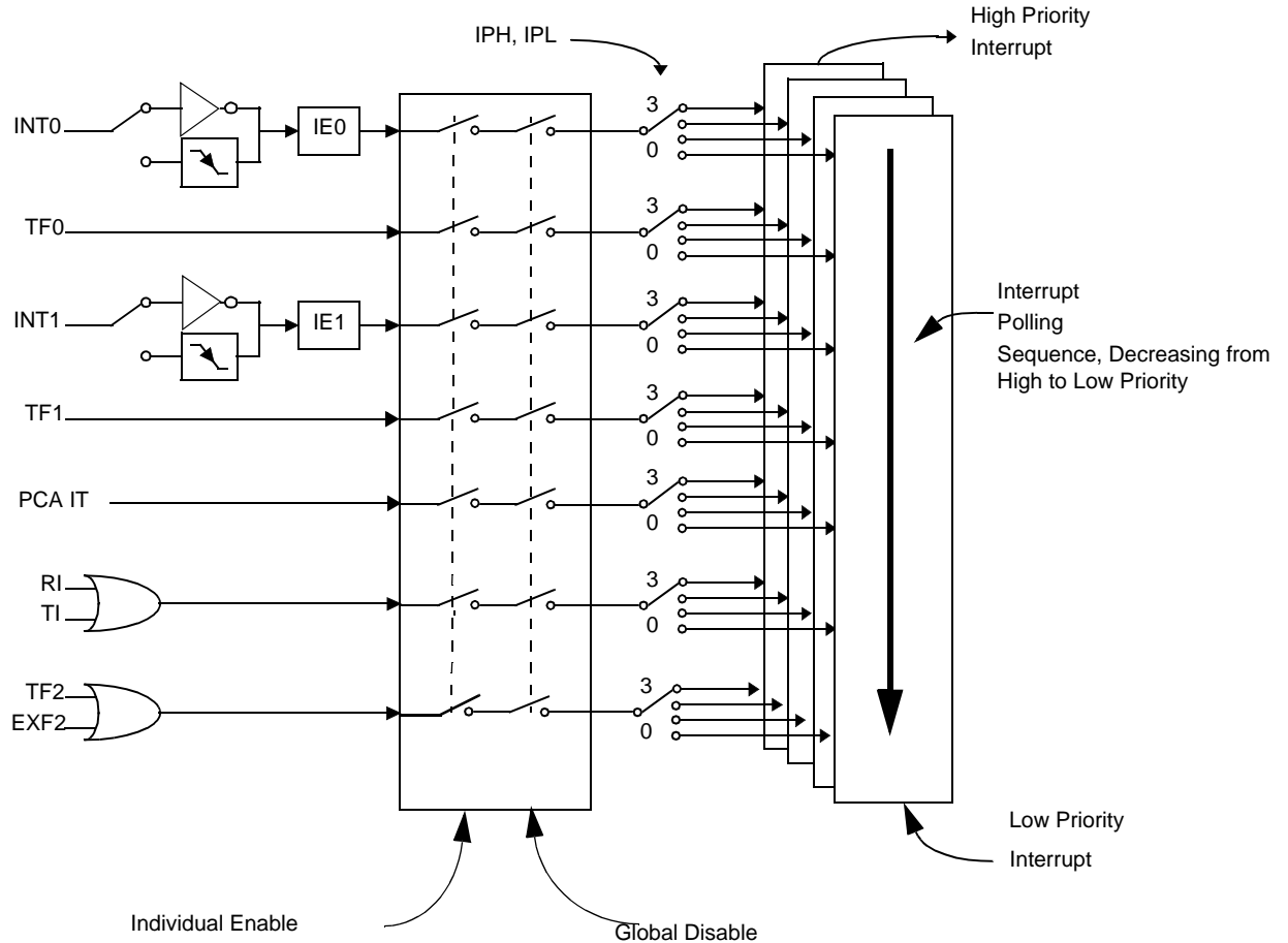
Figure 38. Interrupt Control System
