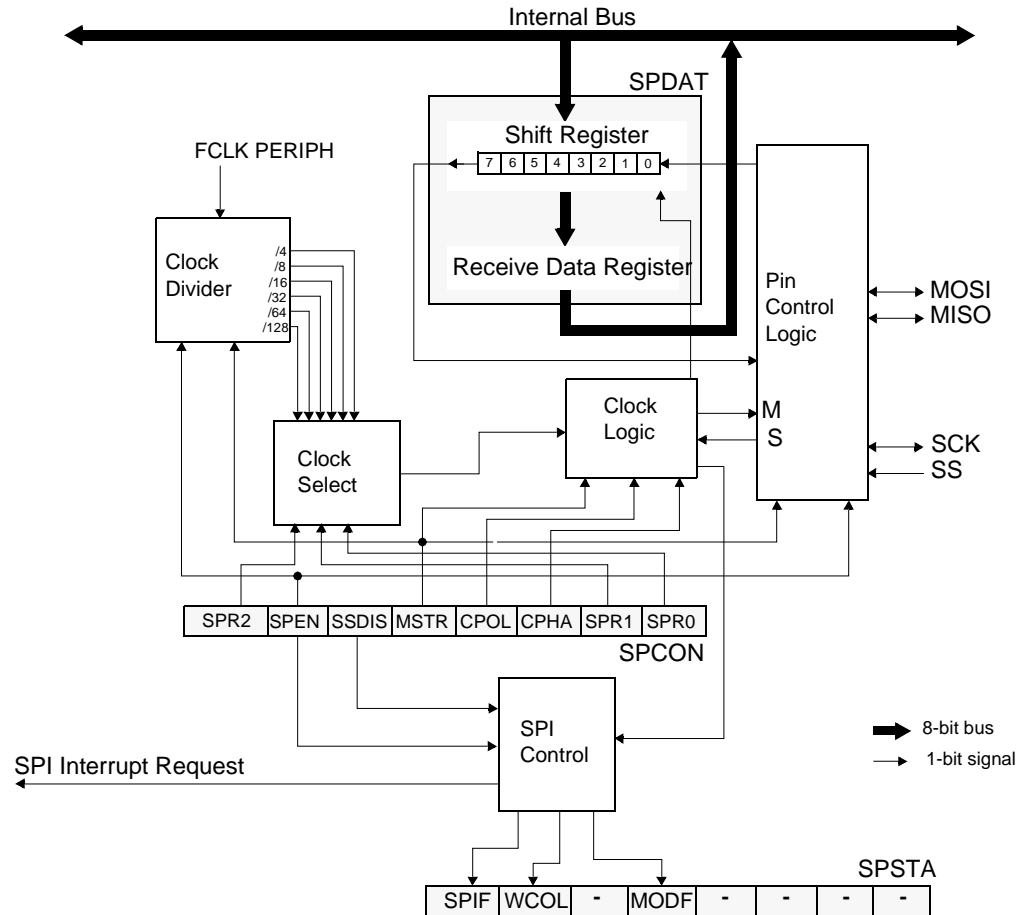
Figure 32. SPI Module Block Diagram
