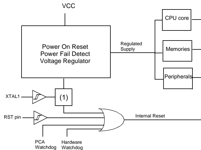
Figure 14. Power Monitor Block Diagram
