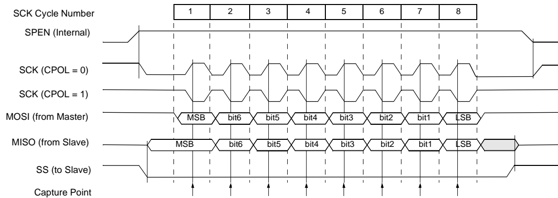
Figure 34. Data Transmission Format (CPHA = 0)
