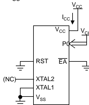
Figure 56. I_{CC} Test Condition, Power-down Mode
