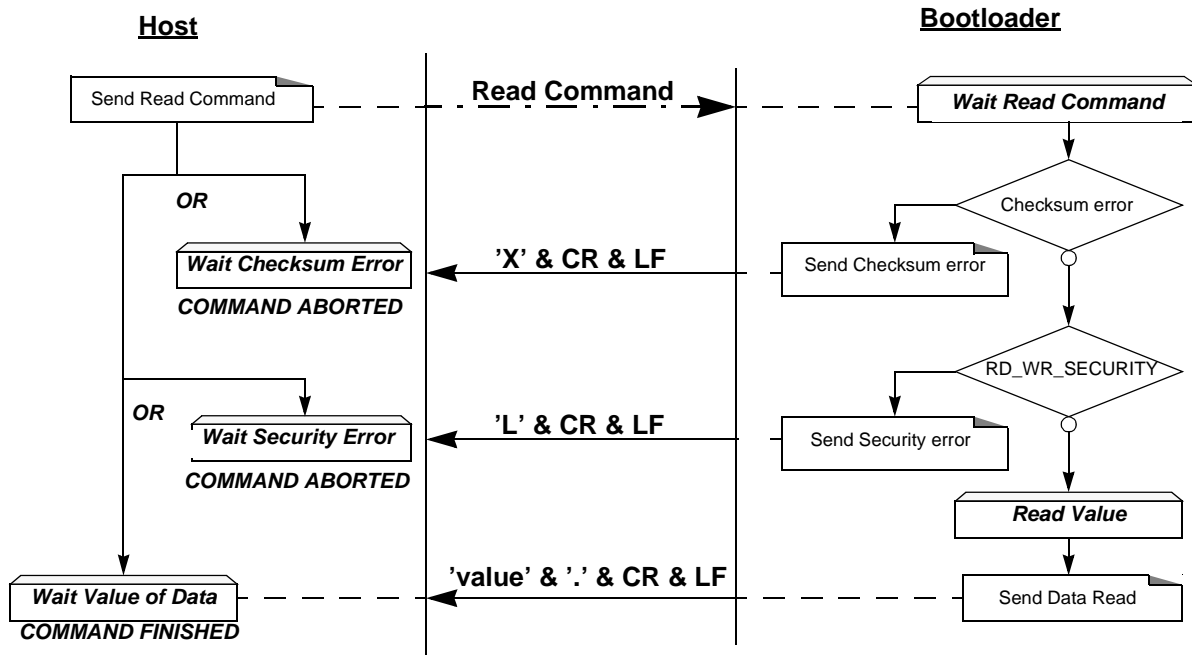
Figure 53. Read Flow
