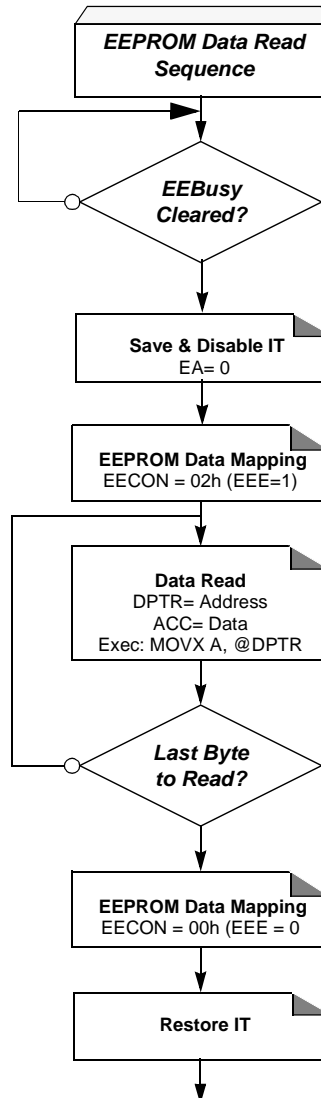
Figure 41. Recommended EEPROM Data Read Sequence
