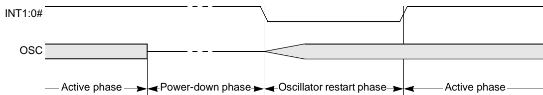
Figure 39. Power-Down Exit Waveform Using INT1:0#
