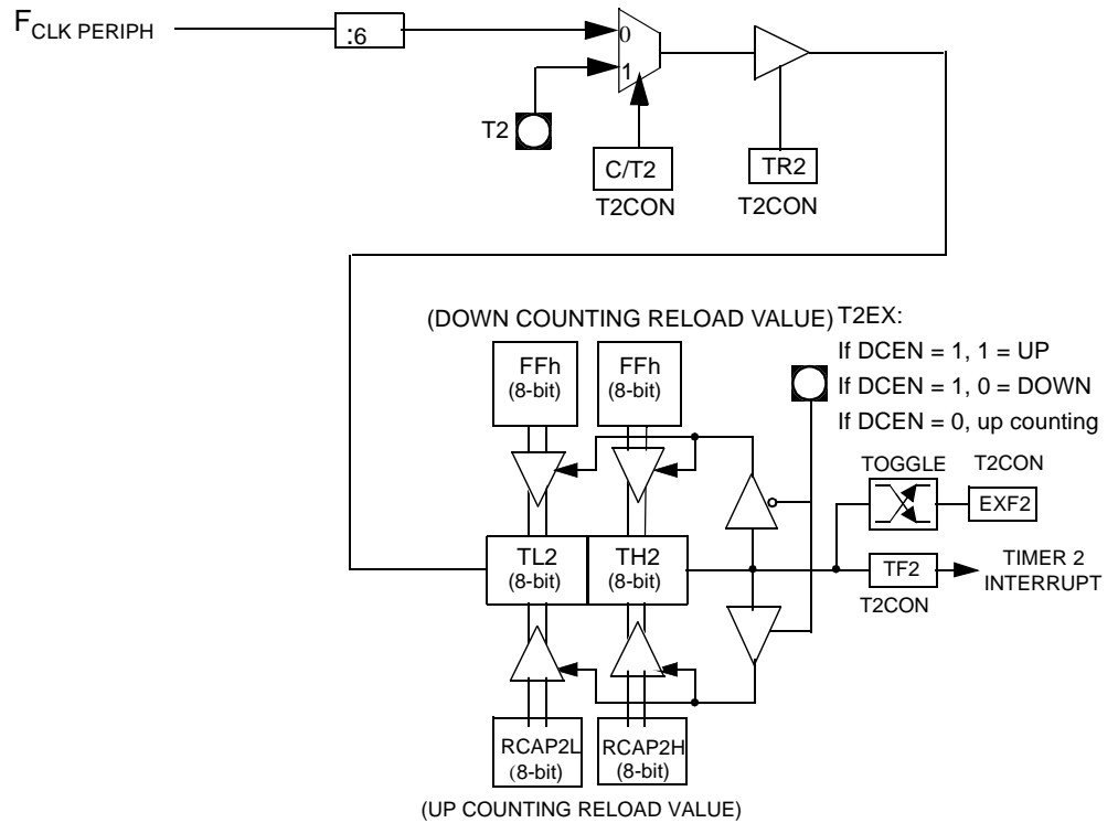
Figure 16. Auto-reload Mode Up/Down Counter (DCEN = 1)
