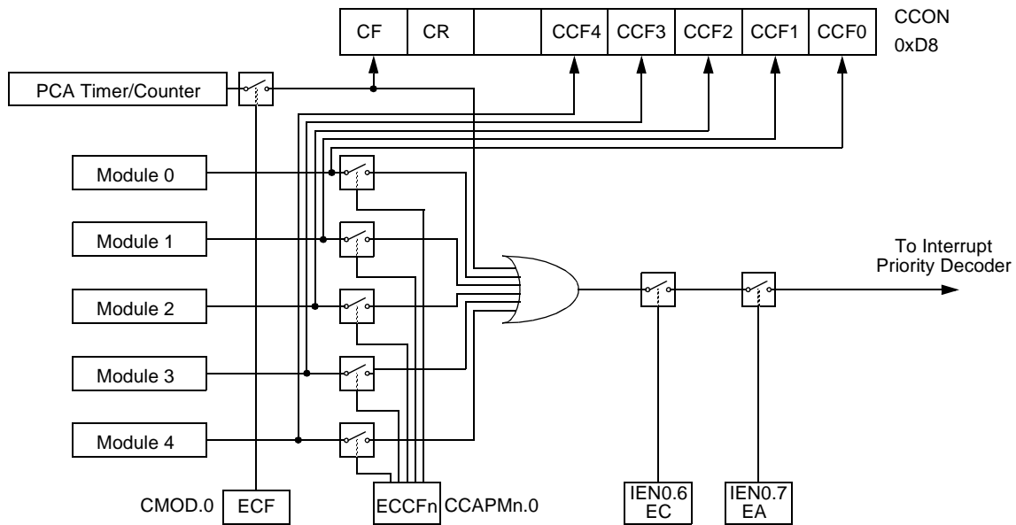
Figure 19. PCA Interrupt System
