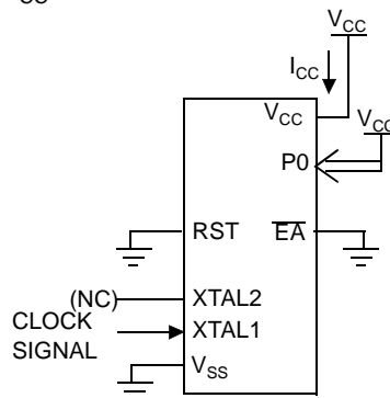
Figure 55. I_{CC} Test Condition, Idle Mode
