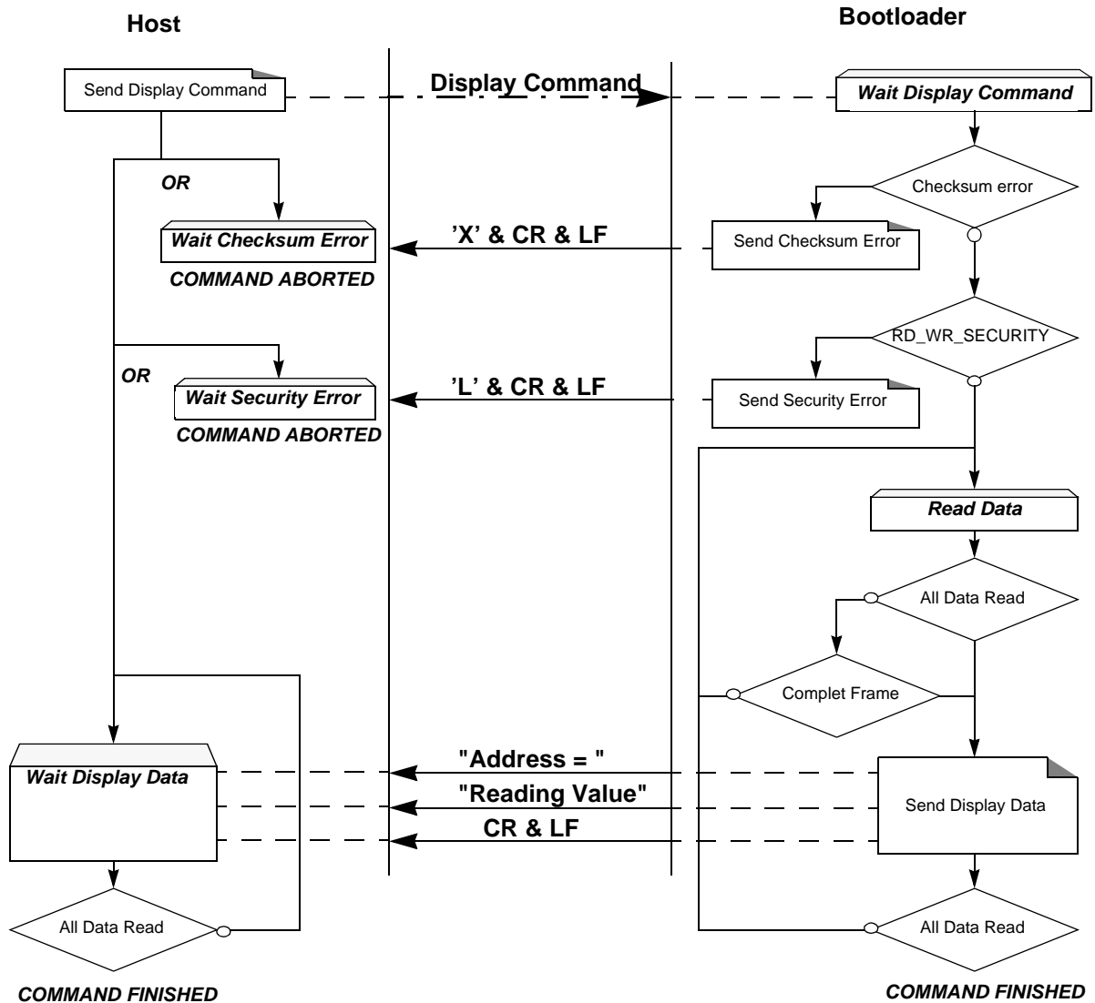
Figure 52. Display Flow
