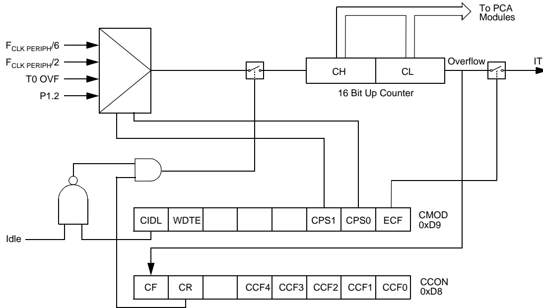
Figure 18. PCA Timer/Counter
