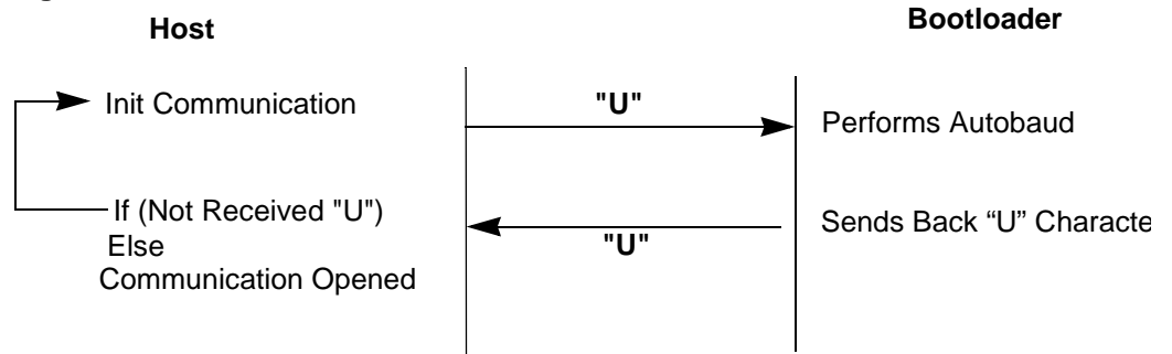
Figure 48. Initialization
