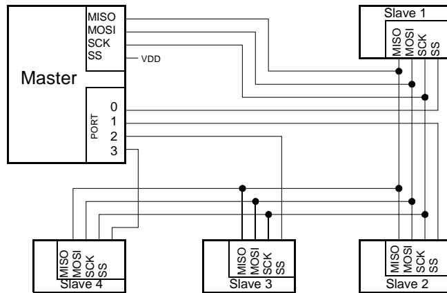
Figure 31. SPI Master/Slaves Interconnection
