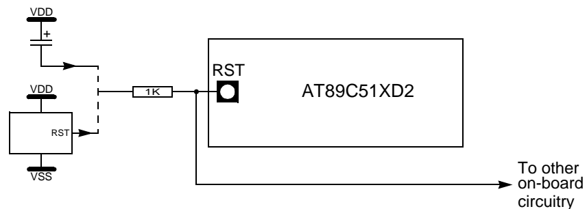
Figure 12. Recommended Reset Output Schematic
