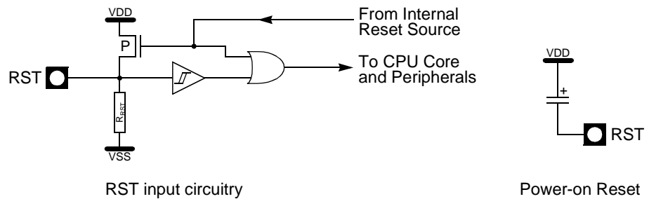
Figure 10. Reset Circuitry and Power-On Reset for AT89S54/58
