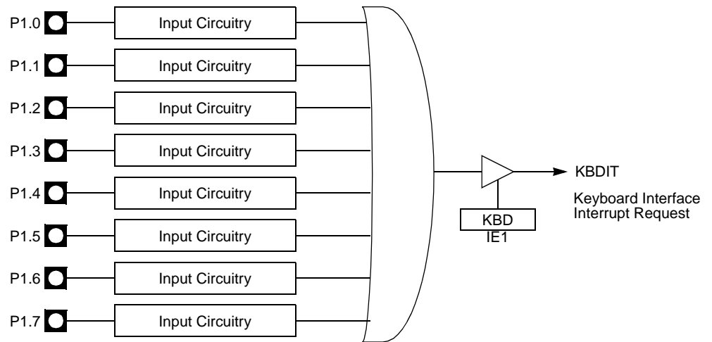
Figure 30. Keyboard Input Circuitry
