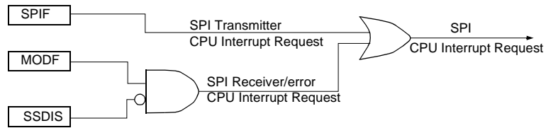
Figure 37. SPI Interrupt Requests Generation
