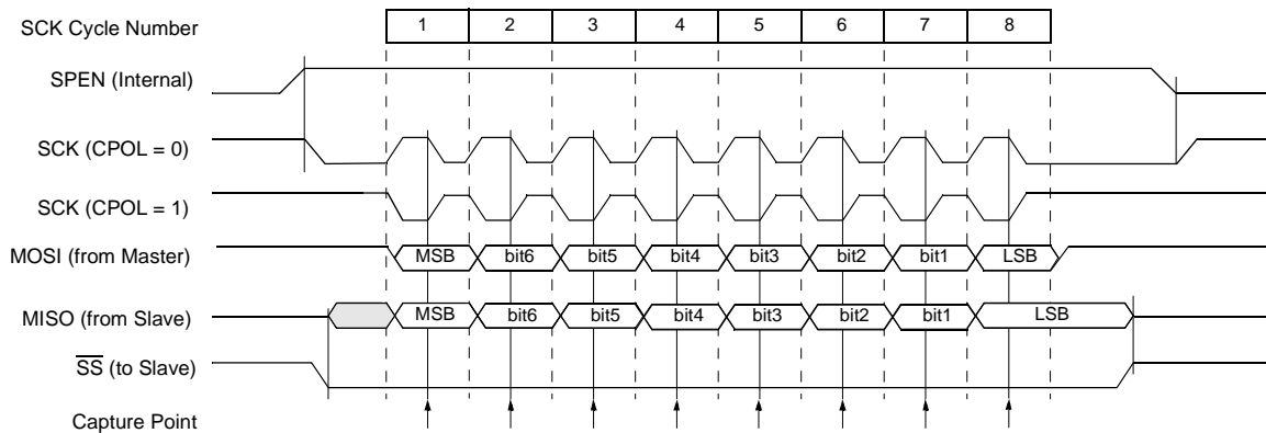
Figure 35. Data Transmission Format (CPHA = 1)
