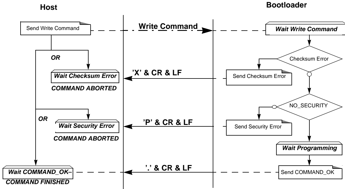
Figure 50. Write/Program Flow
