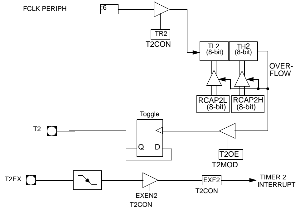
Figure 17. Clock-out Mode C/\overline{T2} = 0
