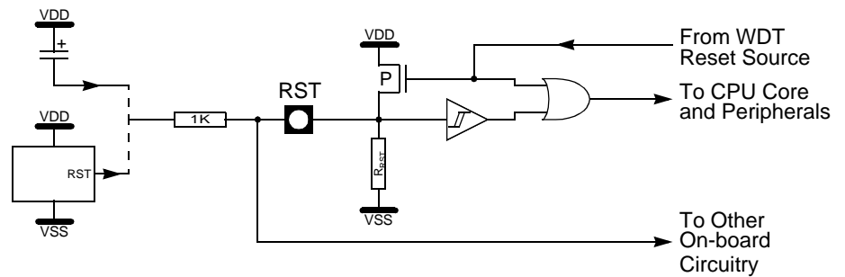
Figure 13. Reset Circuitry for WDT Reset-out Usage
