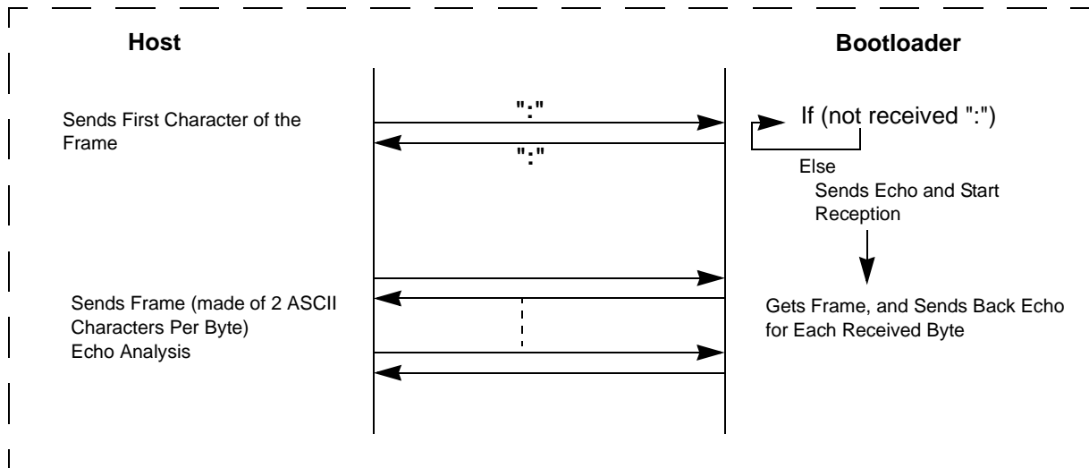
Figure 49. Command Flow
