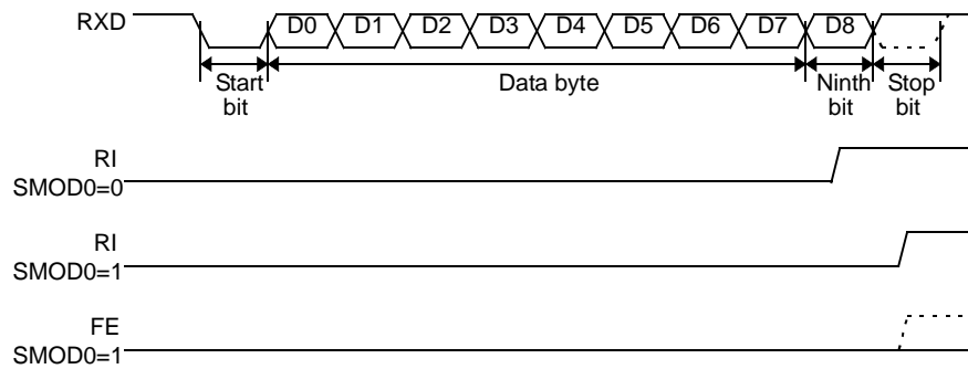
Figure 26. UART Timings in Modes 2 and 3
