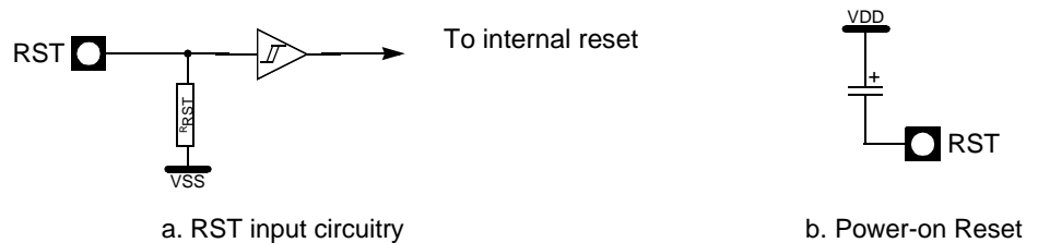
Figure 11. Reset Circuitry and Power-On Reset
