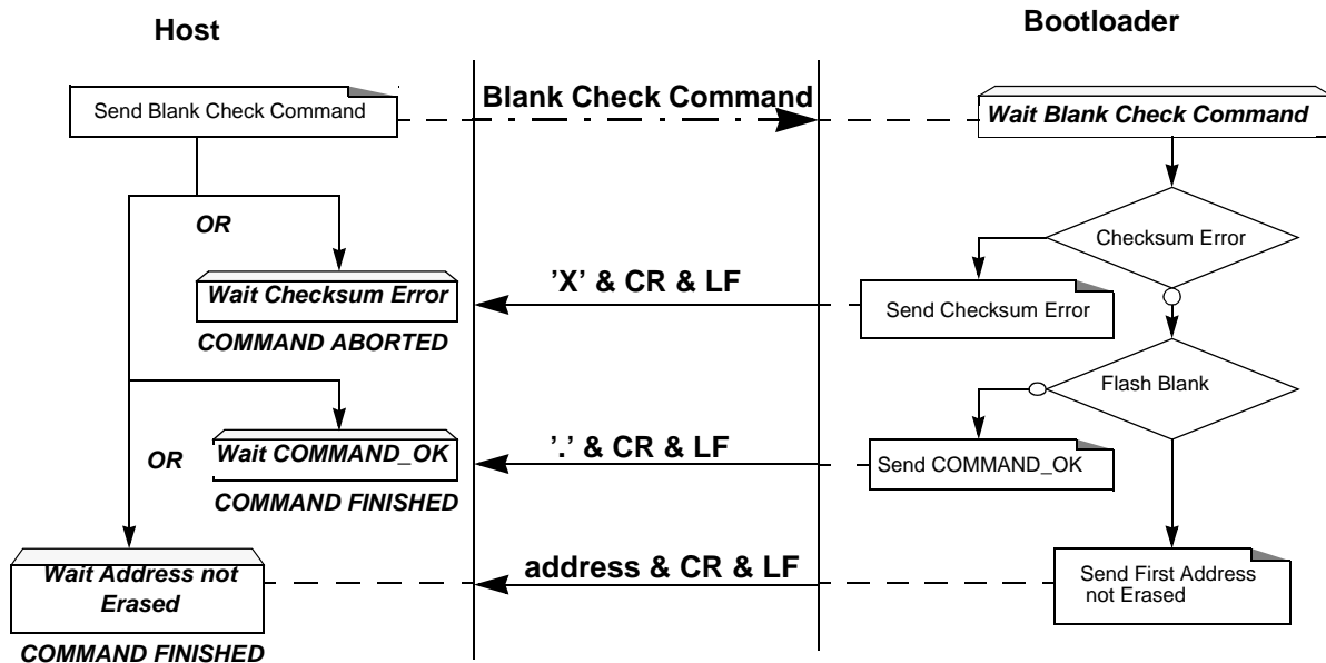
Figure 51. Blank Check Flow
