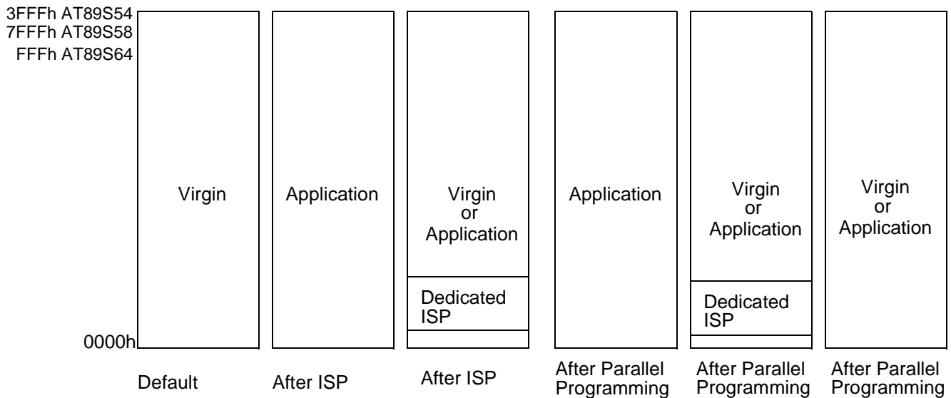
Figure 42. Flash Memory Possible Contents
