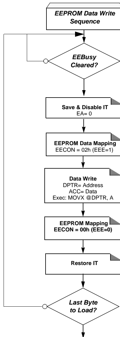
Figure 40. Recommended EEPROM Data Write Sequence
