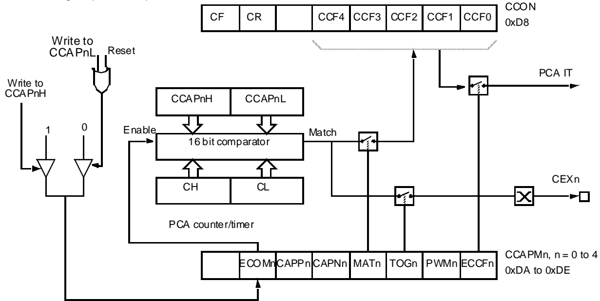
Figure 22. PCA High Speed Output Mode
