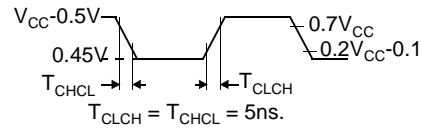
Figure 57. Clock Signal Waveform for I_{CC} Tests in Active and Idle Modes
