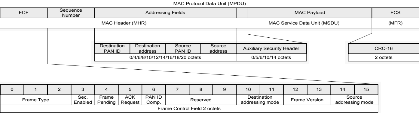
Figure 8-2. IEEE 802.15.4-2006 Frame Format - MAC-Layer Frame Structure (MPDU).
