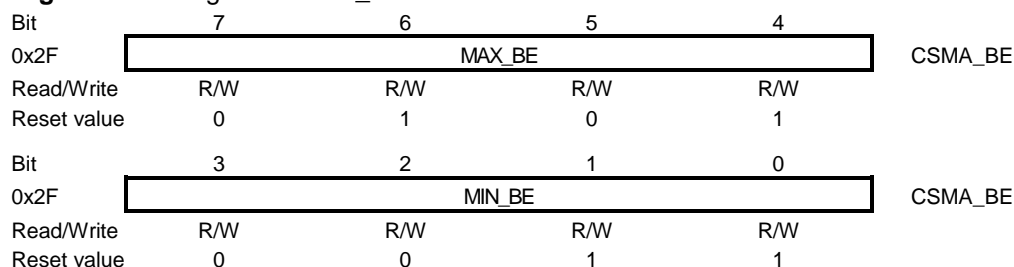
Figure 7-23. Register CSMA_BE.
