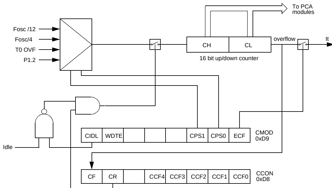
Figure 23. PCA Timer/Counter
