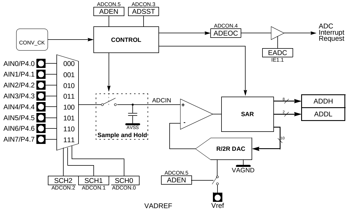
Figure 19. ADC Description
