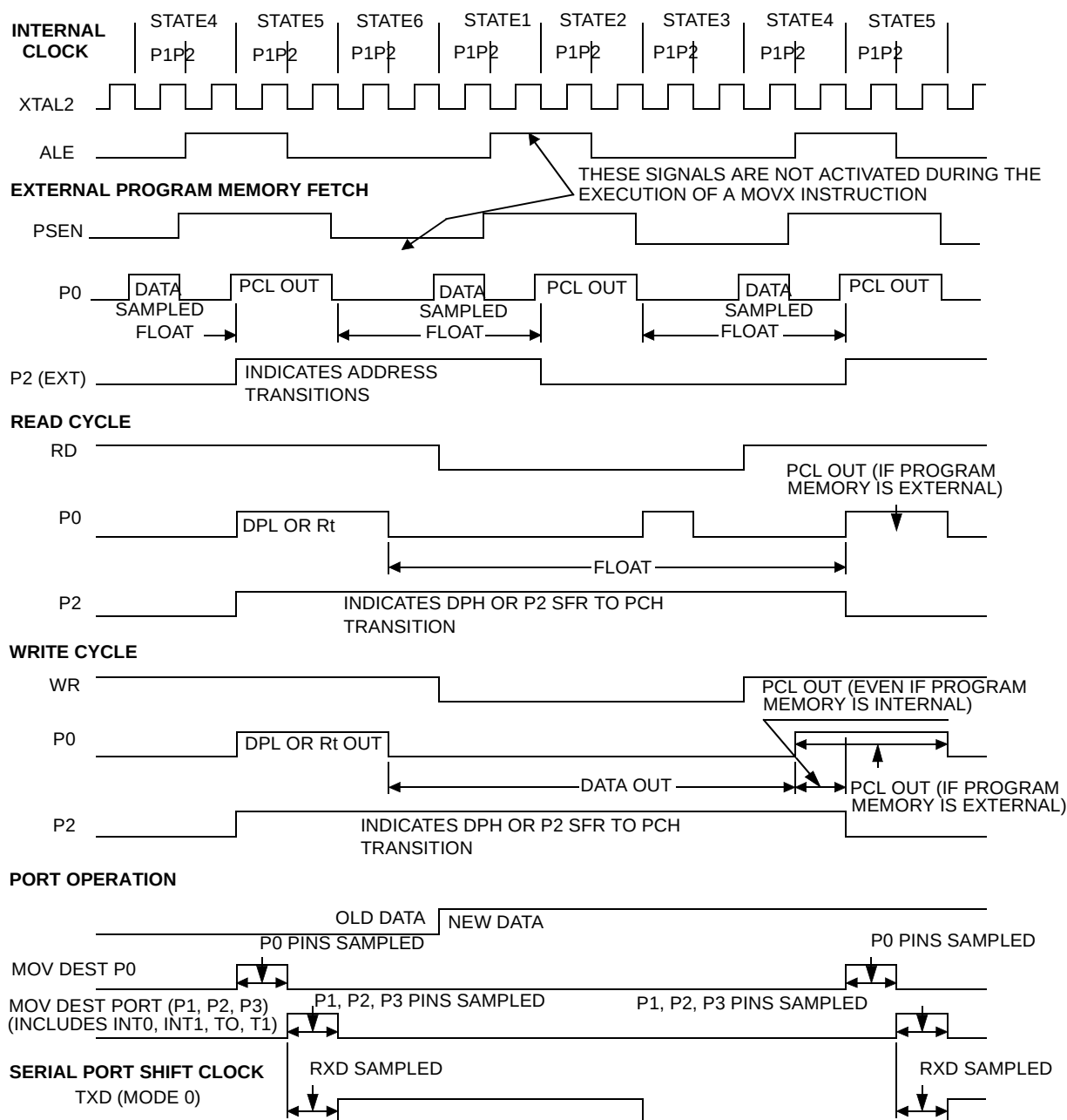
Figure 45. Clock Waveforms
