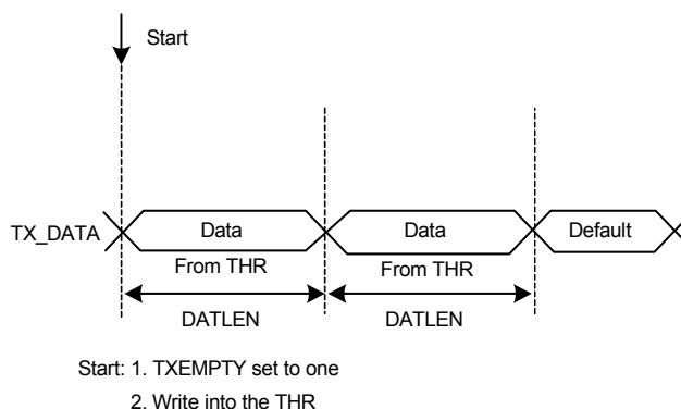
Figure 20-14. Transmit Frame Format in Continuous Mode
