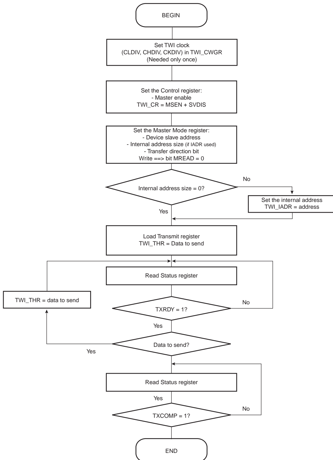
Figure 19-16. TWI Write Operation with Multiple Data Bytes with or without Internal Address
