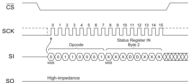
Figure 11-3. Write Status Register Byte 2
