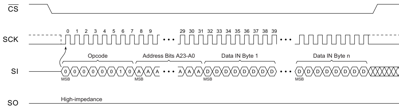
Figure 8-2. Page Program
