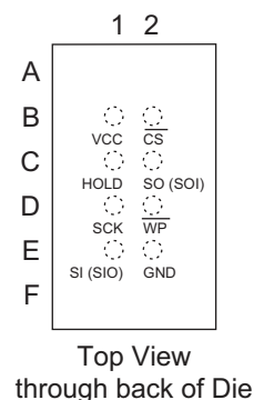
Figure 2-3. 8-ball dBGAs
