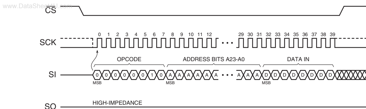
Figure 8-1. Byte Program
