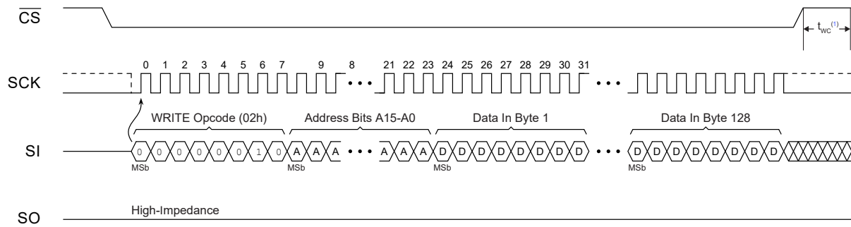
Figure 8-2. Page Write
