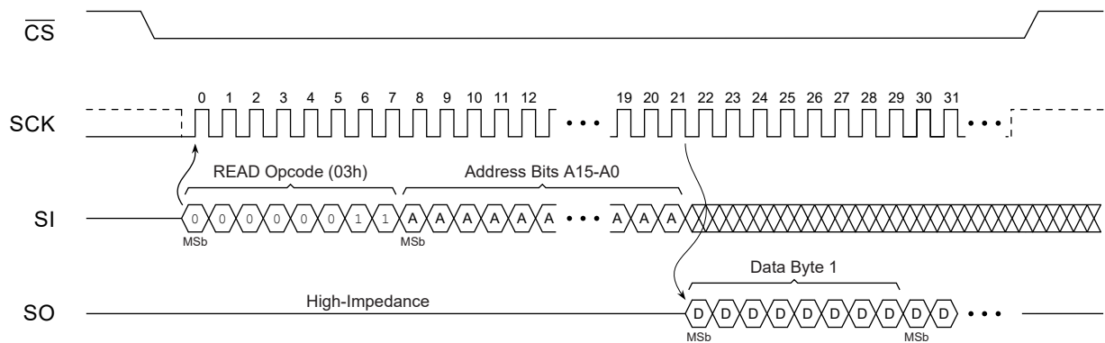
Figure 7-1. Read Waveform
