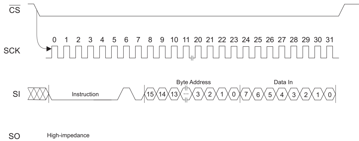
Figure 7-7. Write Timing
