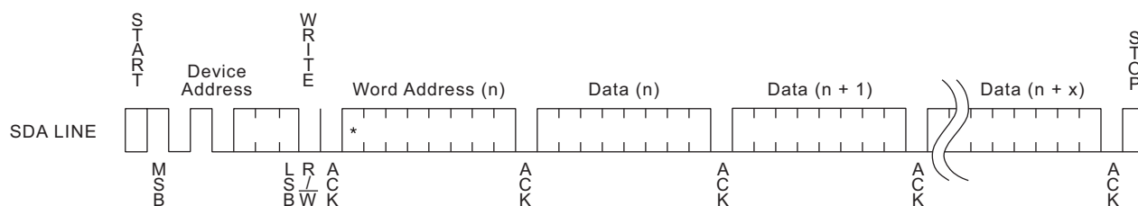
Figure 8-2. Page Write
