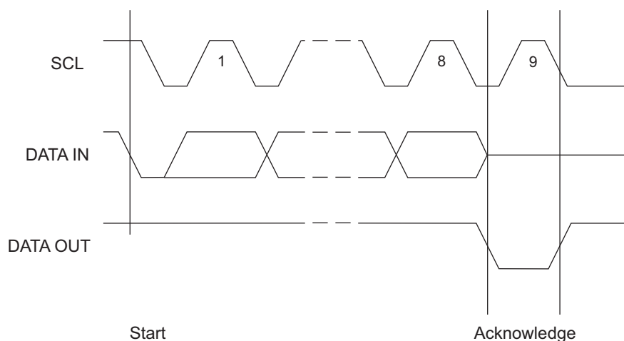
Figure 6-3. Output Acknowledge
