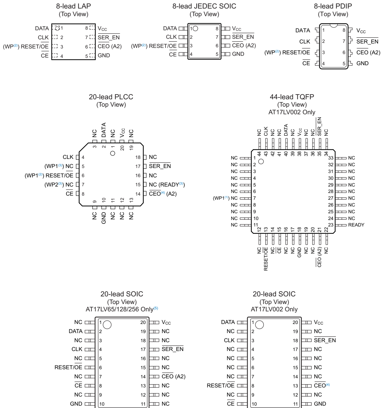
Figure 1-1. Pinouts (1)
