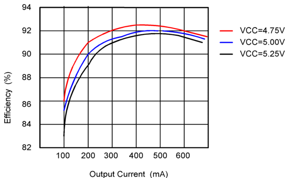
AT1368B Efficiency
