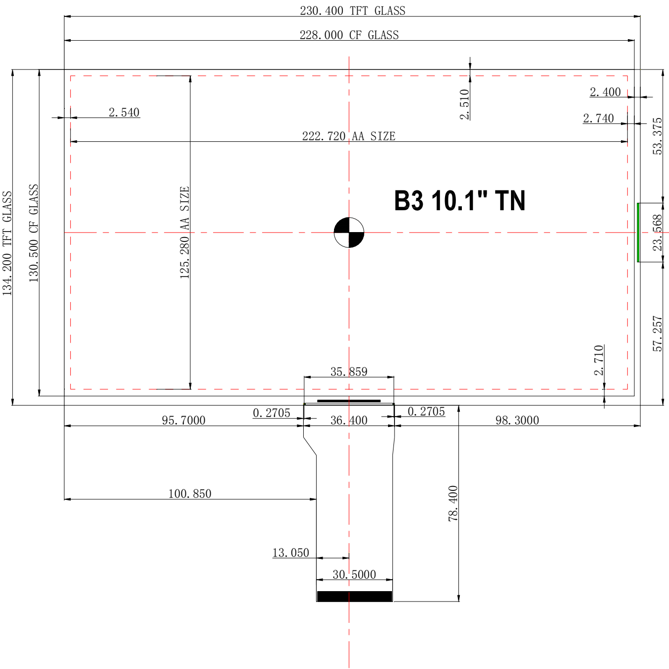
Figure 5. TFT-LCD FOG Outline Dimension
