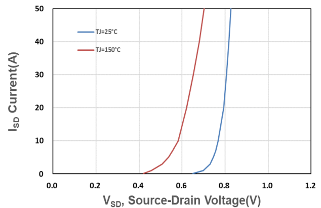
Figure 6. Source-Drain Diode Forward
