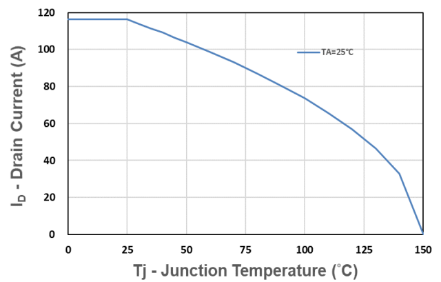
Figure 10. Drain Current
