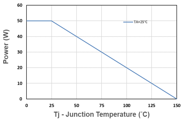
Figure 9. Power Dissipation
