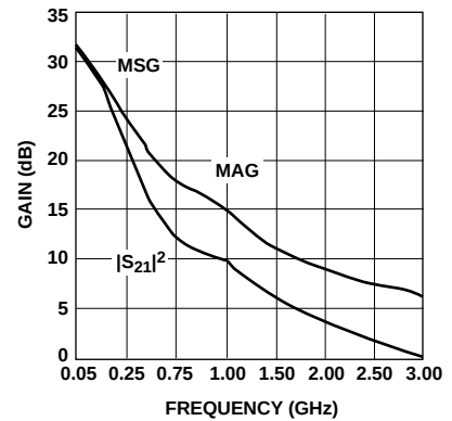
Figure 16. Insertion Power Gain, Maximum Available Gain, and Maximum Stable Gain vs. Frequency. V_{CE} = 6.0V , I_C = 50 mA.
