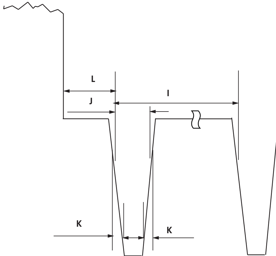
Figure 47: Equivalent Pulse
