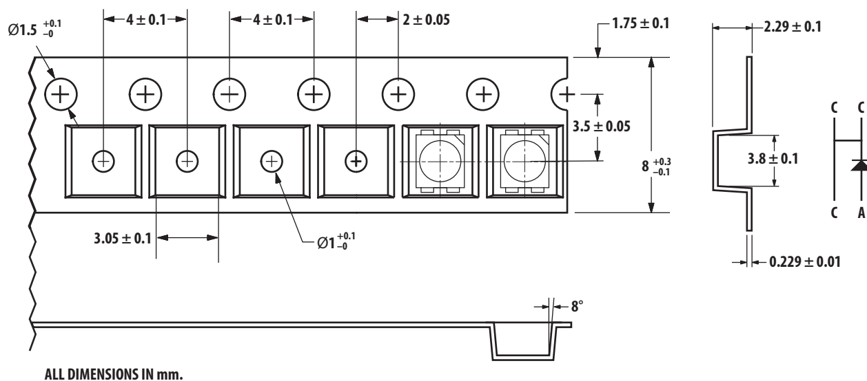
Figure 10. Tape Dimensions
