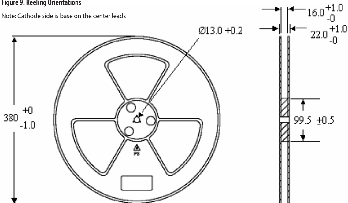
Figure 10. Reel Dimensions
