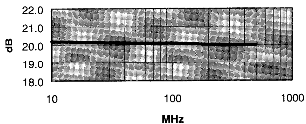
Reverse Isolation vs Frequency
