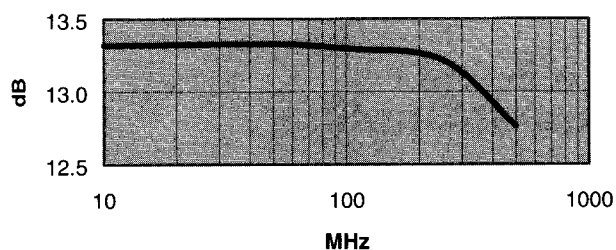
G p vs Frequency
