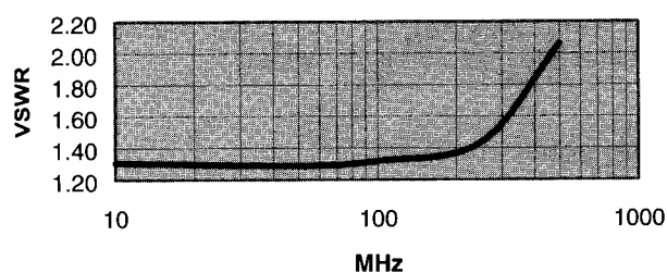
Output VSWR vs Frequency
