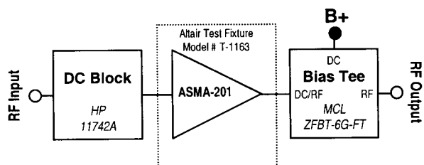
Test Configuration
