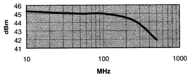
IP 3 vs Frequency
