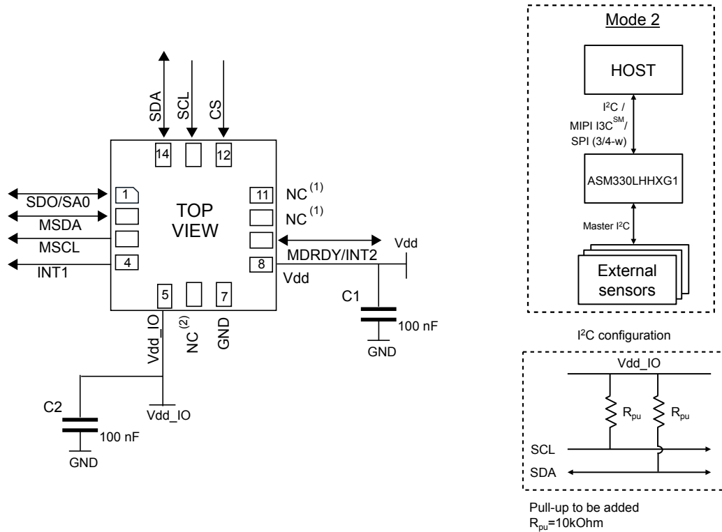
Figure 21. ASM330LHHXG1 electrical connections in mode 2
