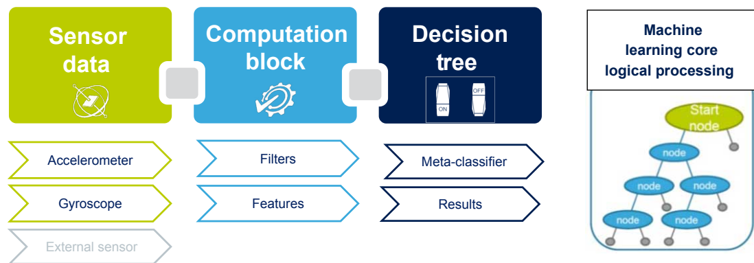
Figure 3. Machine learning core in the ASM330LHHXG1
