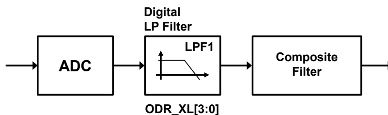
Figure 19. Accelerometer composite filter
