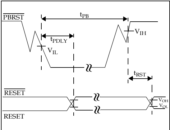
Figure 3: Timing Diagram: Pushbutton Reset
