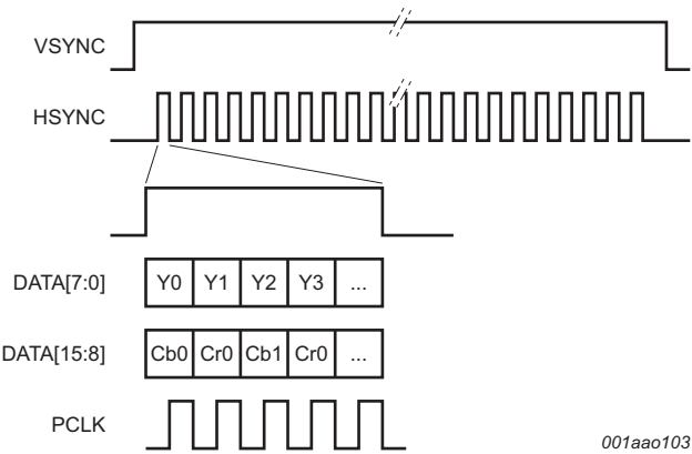
Fig 38. Timing diagram of 16-bit YCbCr with seperate SYNC signals
