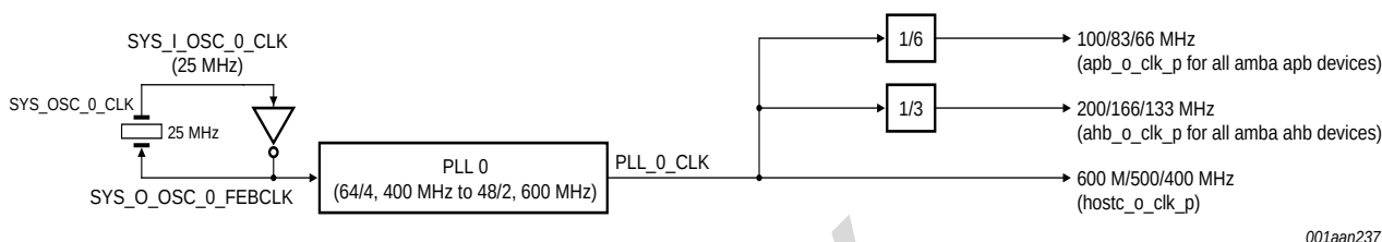
Fig 22. System clock scheme
