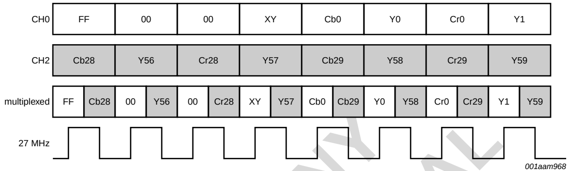
Fig 42. Timing Diagram of Two-Channel Video Stream with Double-Edge Clocking
