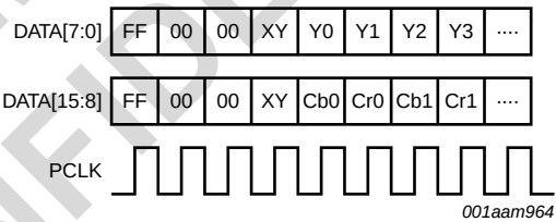
Fig 37. Timing diagram of BT1120
