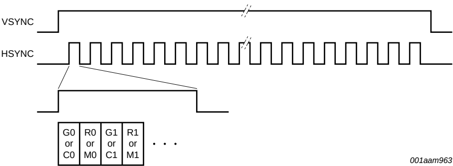
Fig 36. Timing diagram of Bayer RGB and CMYG format
