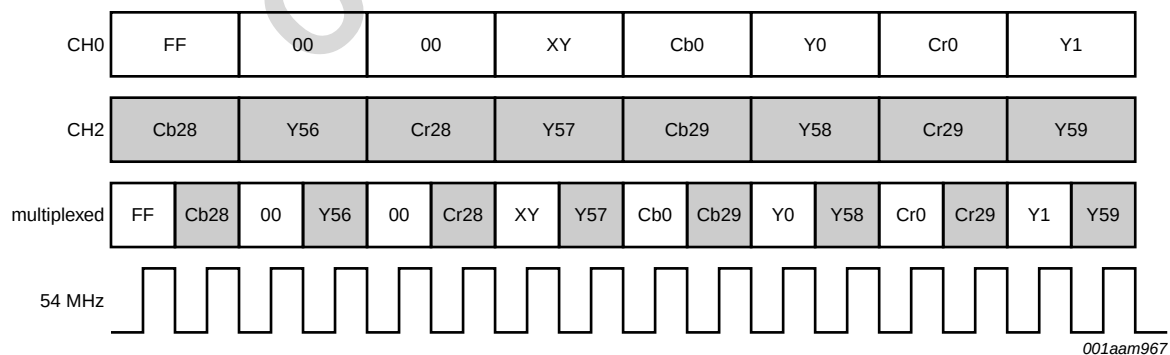
Fig 41. Timing Diagram of Two-Channel Video Stream with Single-Edge Clocking
