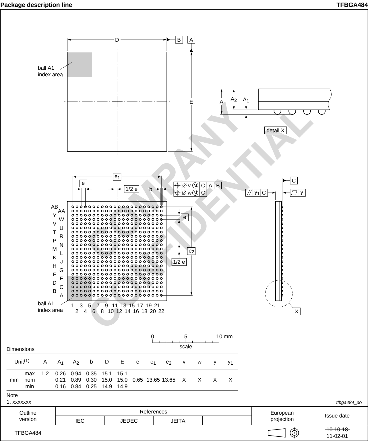
Fig 59. ASC8848/49/50/51 SoC TFBGA-484 Package Physical Dimension
