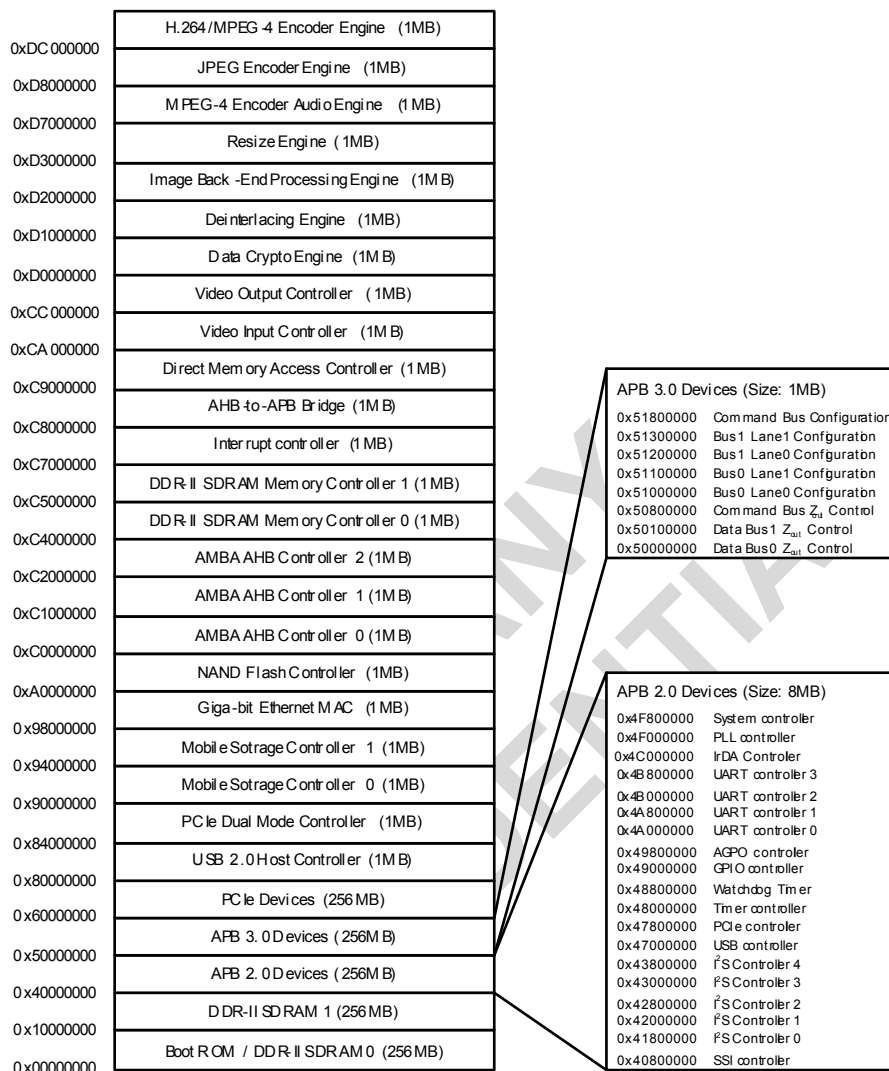
Fig 10. Illustration of Memory Map in ASC8848/49/50 M1 version SoC
