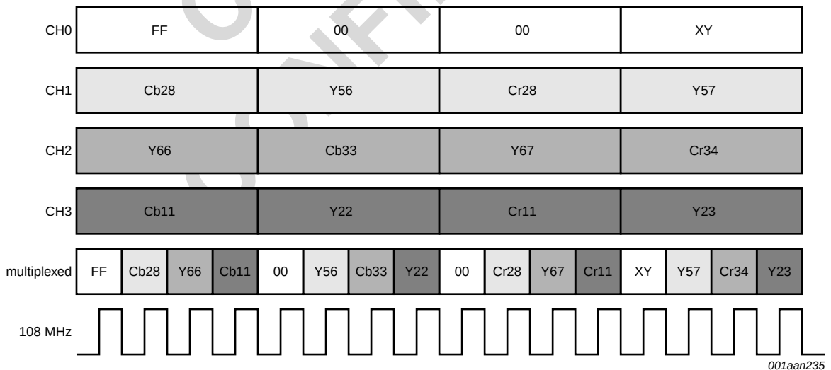
Fig 43. Timing Diagram of Four-Channel Video Stream with Single-Edge Clocking
