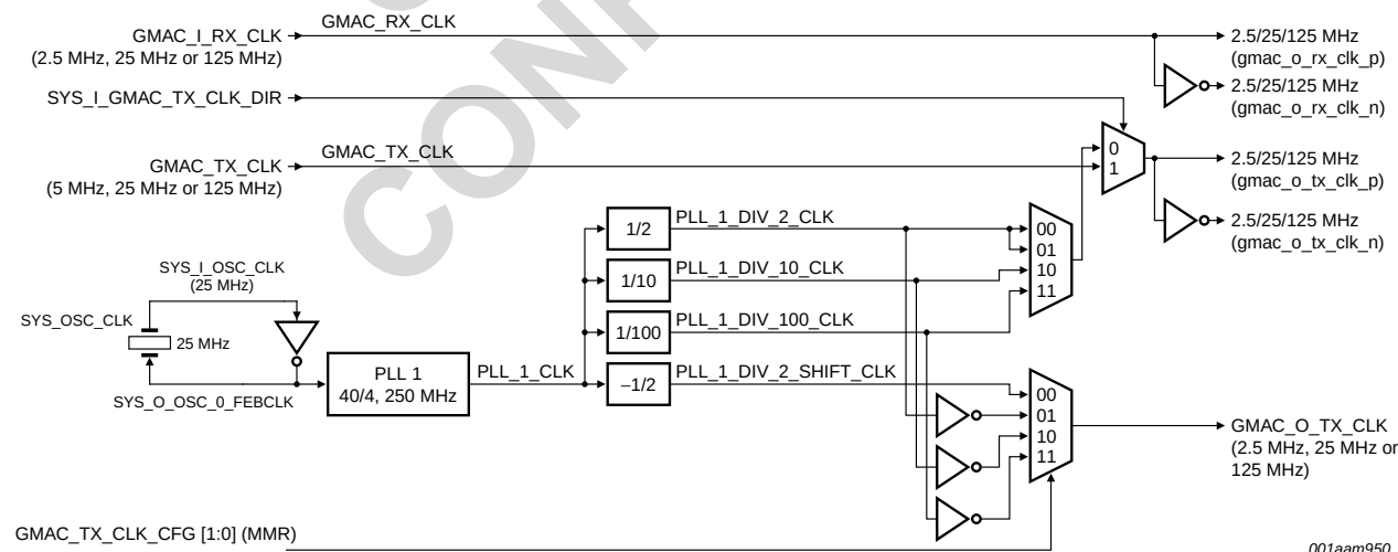
Fig 23. Gigabit Ethernet Clock Scheme (for ASC8850/49/48 M1)
