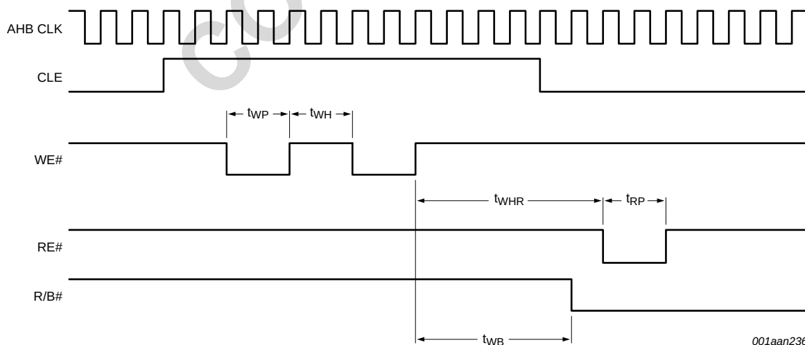
Fig 51. Timing relationship
