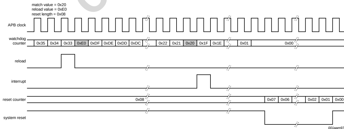
Fig 53. Operation of the Watchdog Timer
