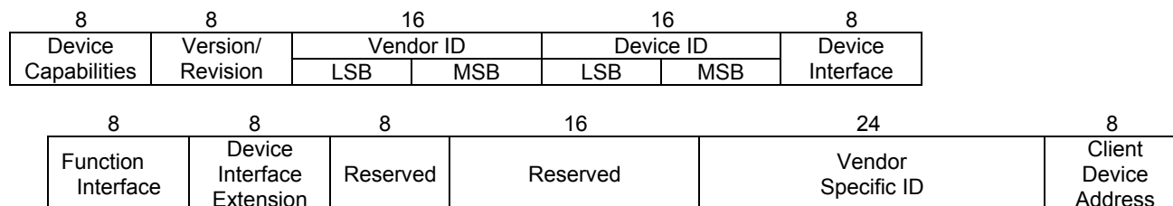
Figure 13. Device Identifier Block
