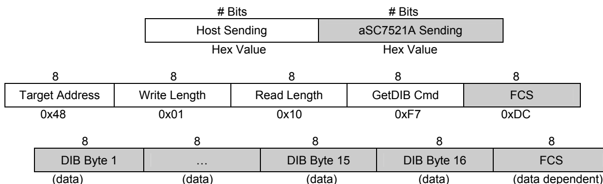
Figure 3. GetDIB() Command (16-byte read length)
