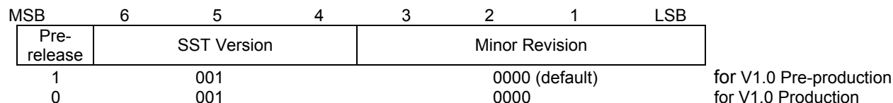
Figure 15. Version / Revision Field
