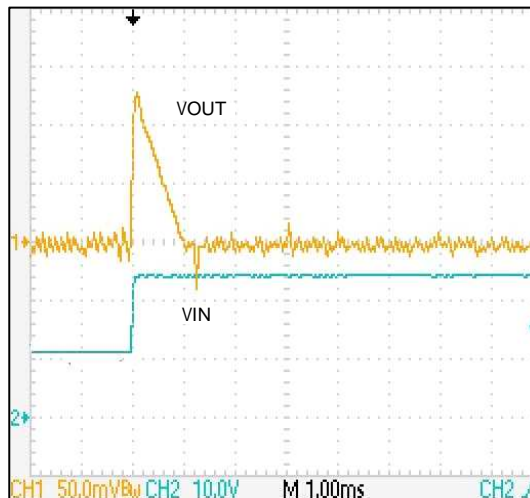
Figure 14. Line Regulation VOUT=5V @ 10mA
