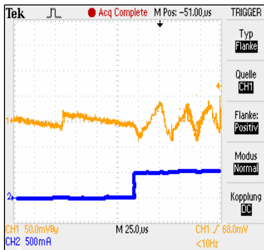
Figure 16. Load Regulation VOUT=5V 10mA→500mA
