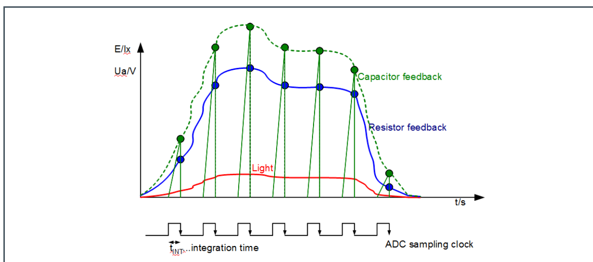
Figure 38: Difference Between Resistive and Capacitive Feedback
