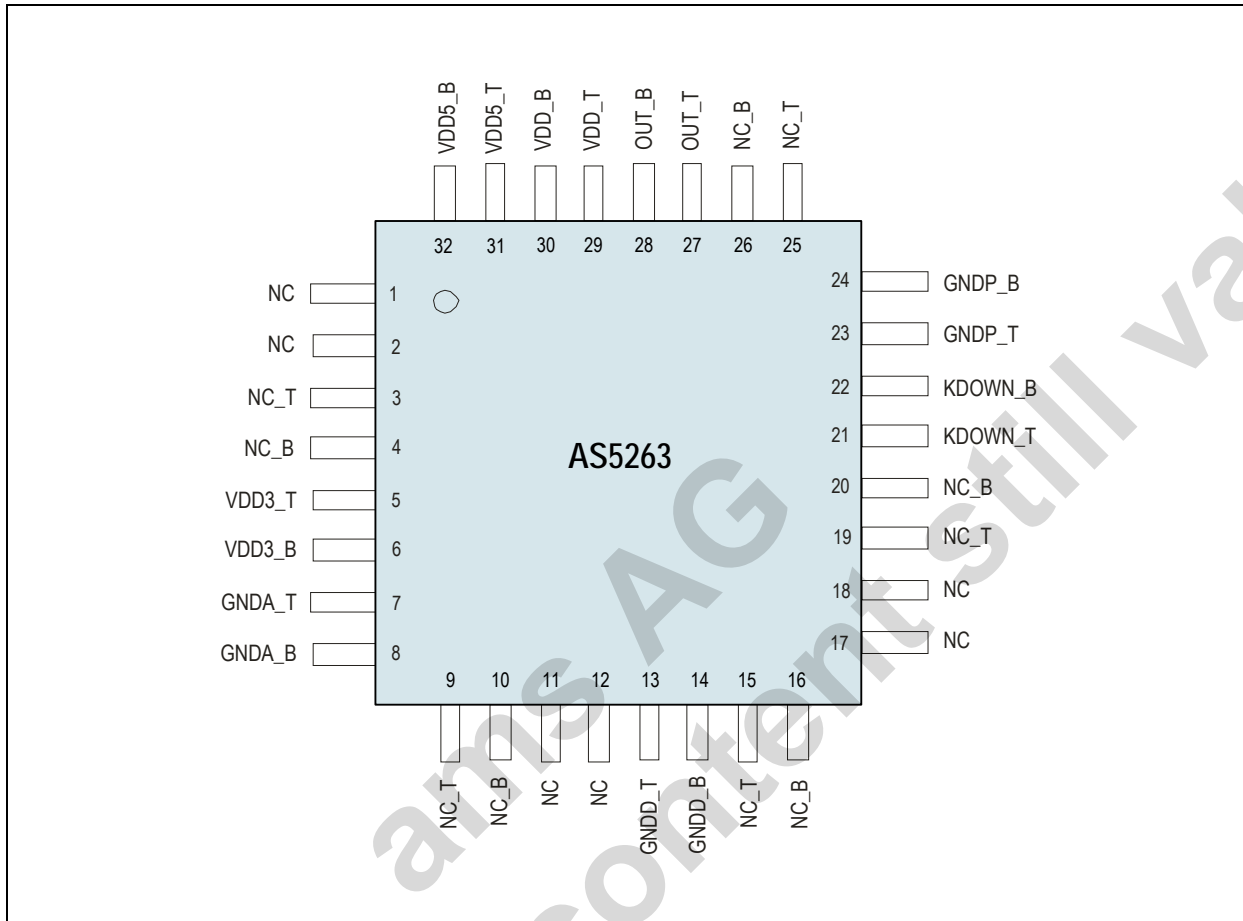
Figure 2. Pin Assignments (Top View)
