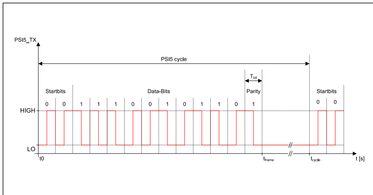
Figure 56: Timing Asynchronous Modes A10P- 50/1L and A10P-500/1L
