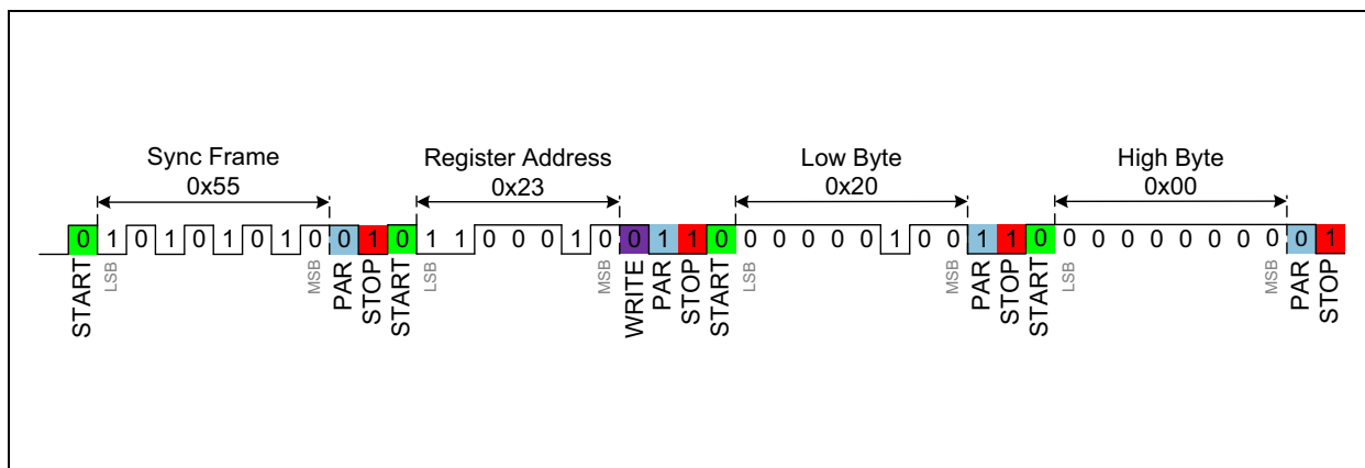
Figure 27: Example of WRITE (Reg[0x23] = 0x20 and Reg [0x24] = 0x00)
