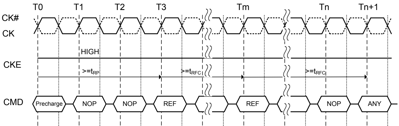
Figure 46. Refresh command
