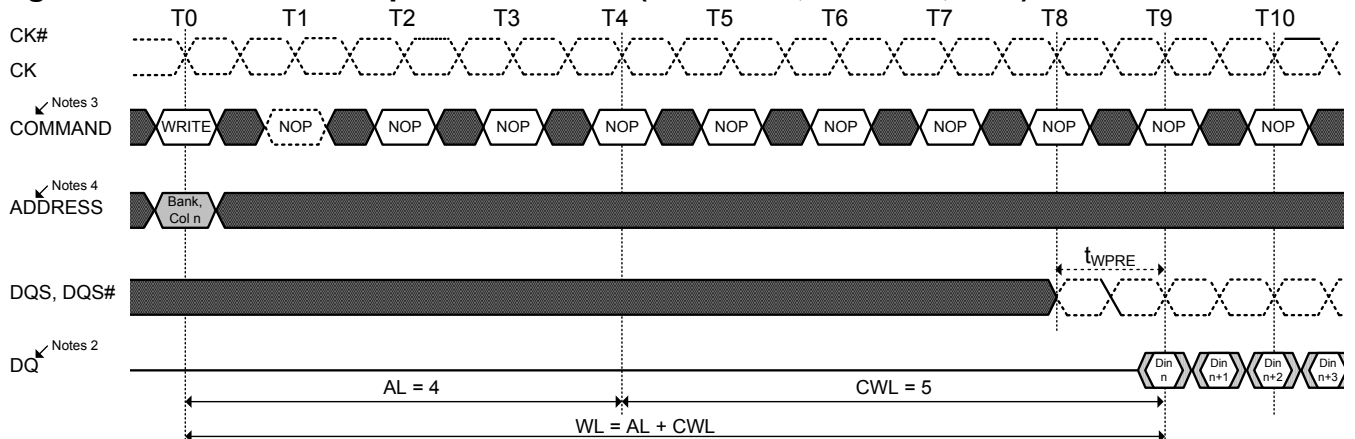
Figure 44. WRITE Burst Operation WL = 9 (AL = CL-1, CWL = 5, BL8)
