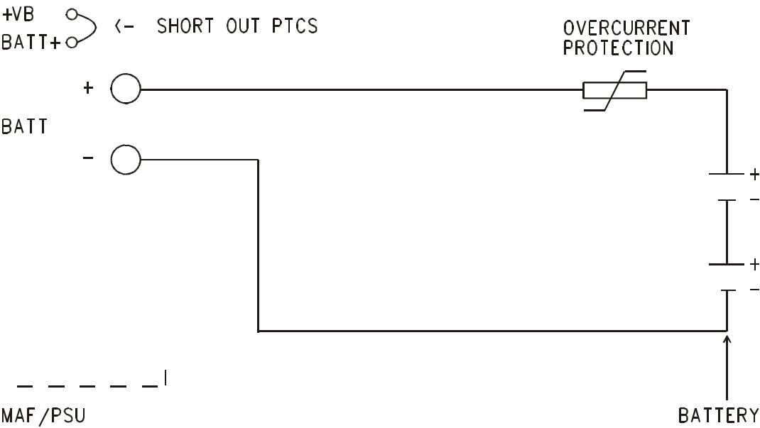
FIG 4.3.2 BATTERY OVERCURRENT PROTECTION FOR LOADS GREATER THAN 3A
