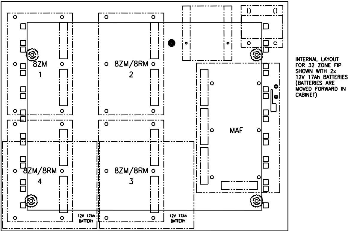
FIG 2.2.2 F3200 SMALL CABINET, MAXIMUM CONFIGURATION
