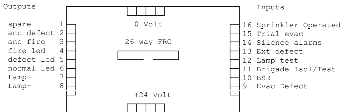
FIG 5.12.3 Terminations from NZ mode Display Extender Board on unprotected termination board (PA0483).
