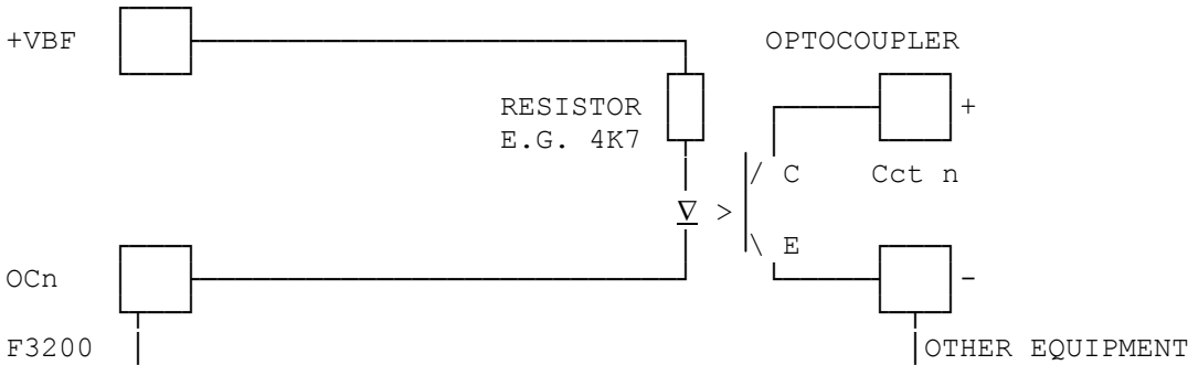
FIG 5.7.3 EXAMPLE OF INTERFACING TO OTHER EQUIPMENT, OPTICAL ISOLATION
