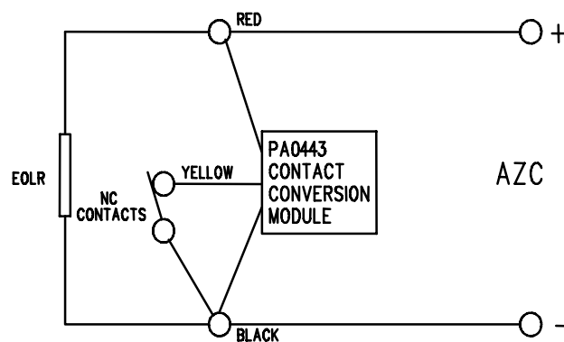
FIG 6.5.1 NORMALLY CLOSED CONTACT WIRING TO F3200 AZC
