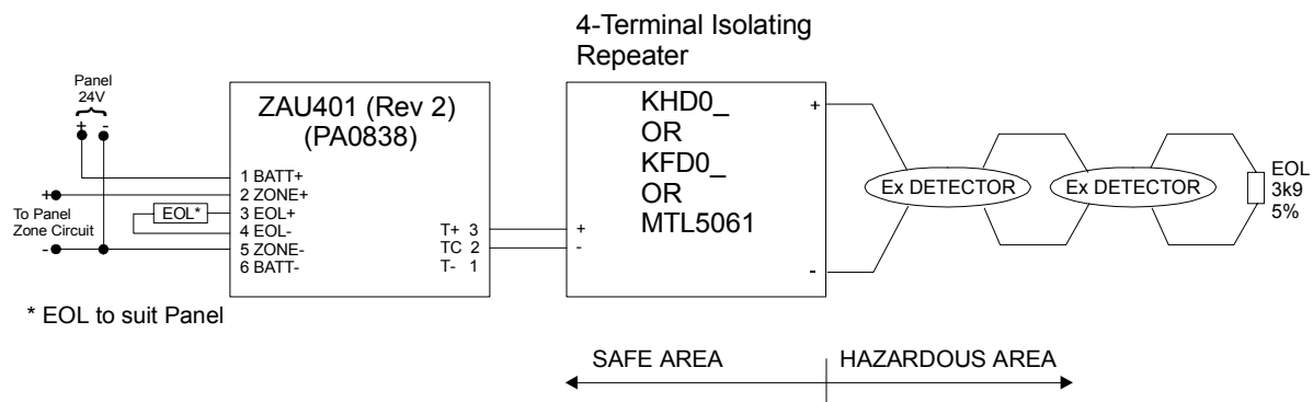
FIG 6.4.3.3 F3200 WITH ZAU401 & 4 TERMINAL IS REPEATER
