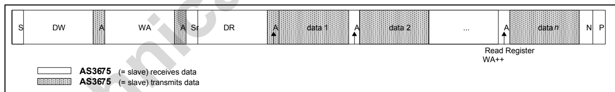
Figure 39. Serial Interface Sequential Read
