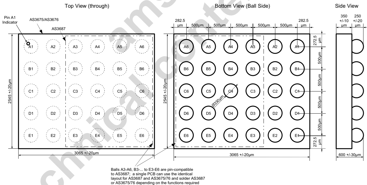
Figure 43. WL-CSP30 3x2.5mm 6x5 Balls Detail Dimensions
