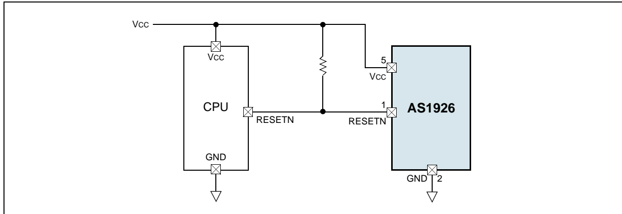
Figure 11. Interfacing to Microprocessors with Bidirectional Reset Pins
