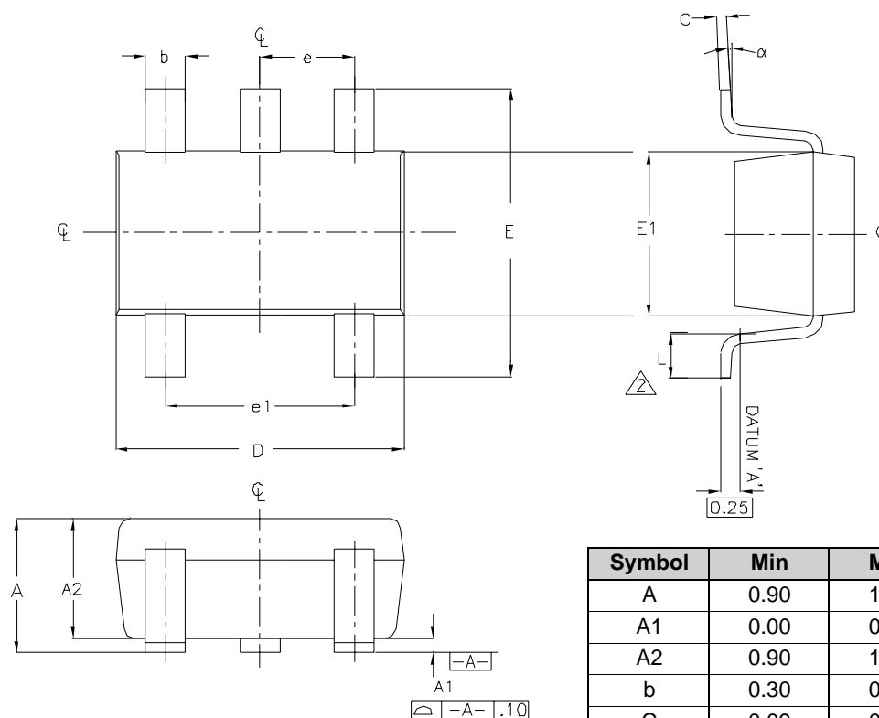
Figure 18. 5-pin SOT23 Package
