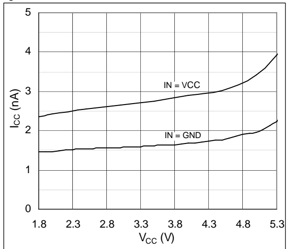
Figure 12. I_{CC} vs. V_{CC}
