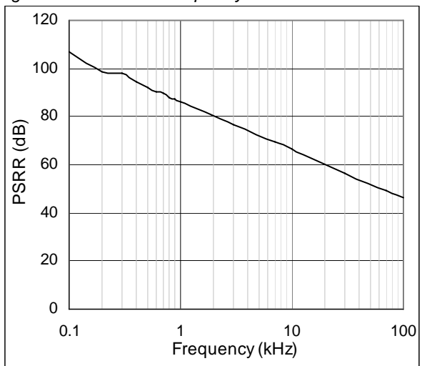
Figure 14. PSRR vs. Frequency
