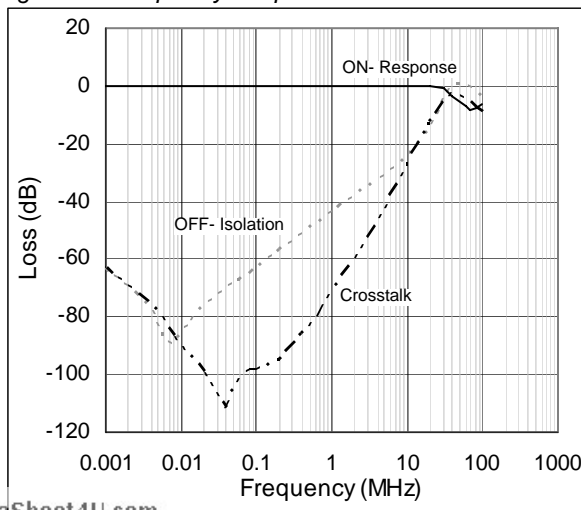
Figure 7. Frequency Response
