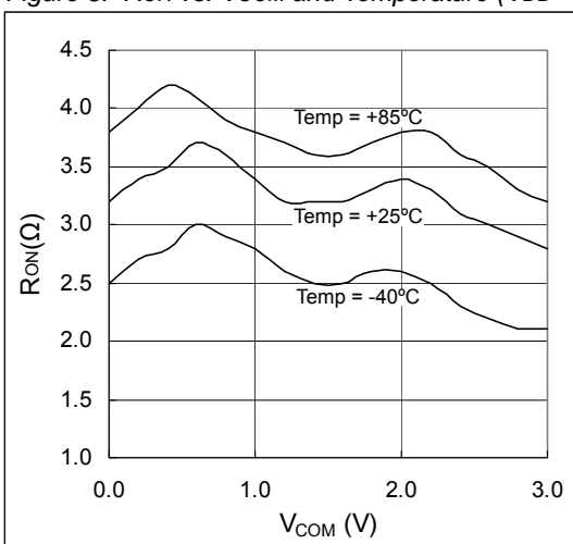
Figure 5. R_{ON} vs. V_{COM} and Temperature ( V_{DD} = 3V )
