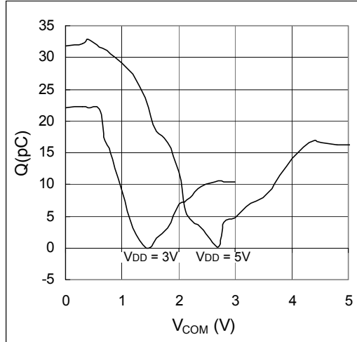
Figure 9. Charge Injection
