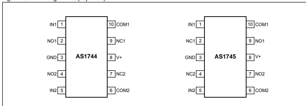
Figure 16. Pin Assignments (Top View)
