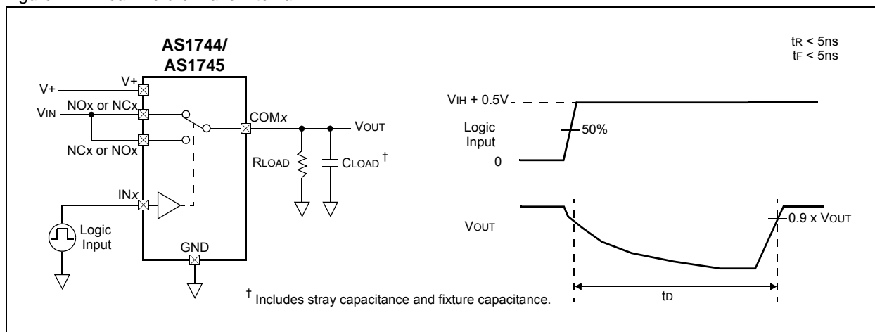
Figure 12. Break-Before-Make Interval
