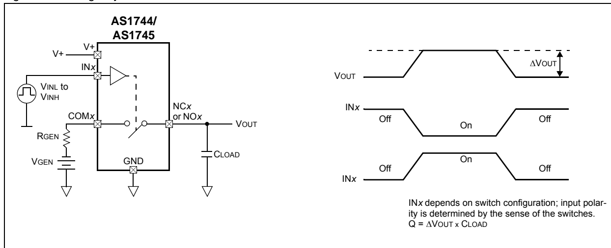
Figure 13. Charge Injection
