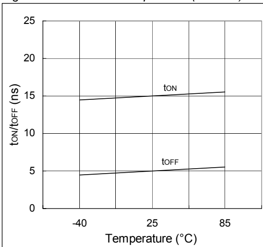
Figure 7. t_{ON}/t_{OFF} vs. Temperature ( V_{+} = 5V )
