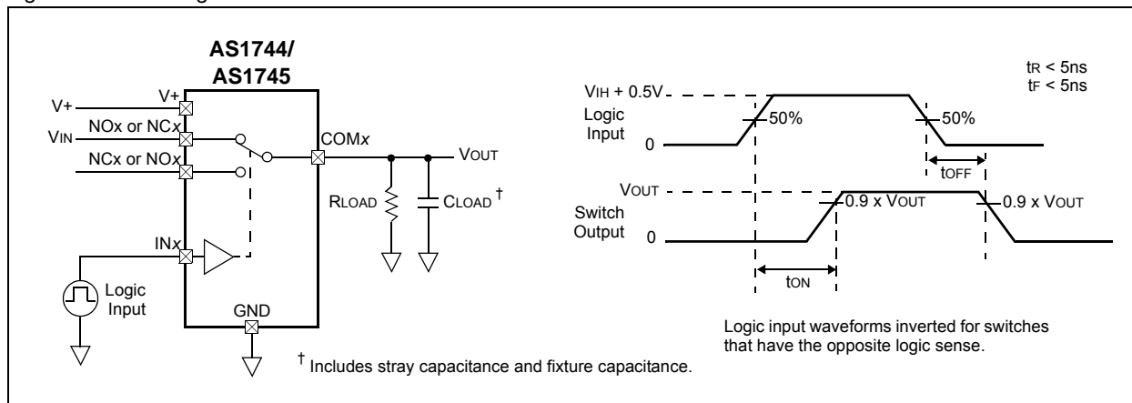
Figure 11. Switching Time
