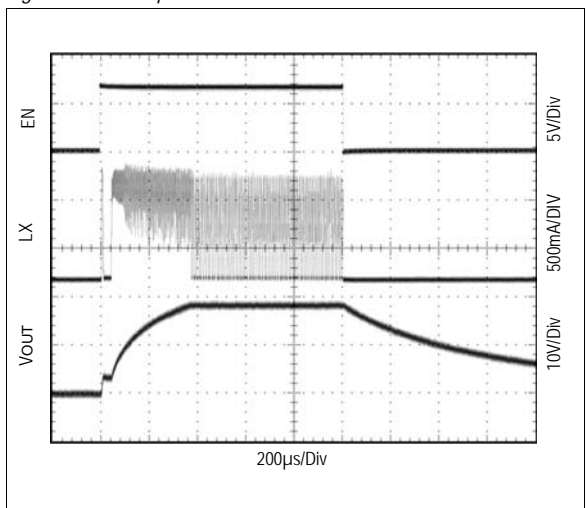
Figure 19. Startup Waveform
