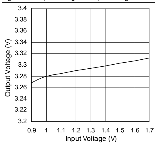
Figure 8. Output Voltage vs. Input Voltage
