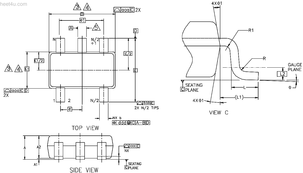
Figure 13. TSOT23-5 Package
