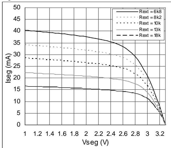
Figure 13. I_{SEG} vs. V_{SEG} ; V_{DD} = 3.3V
