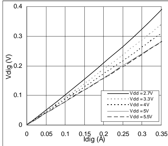
Figure 9. V_{DIGIT} vs. I_{DIGIT}
