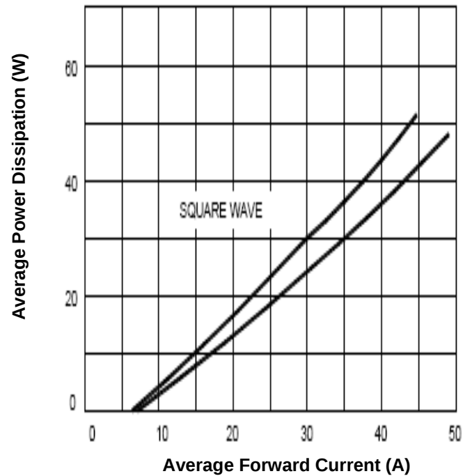
Fig.4-Forward Power Dissipation
